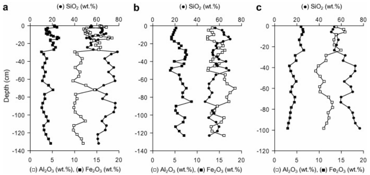
Fig. 4. Concentration (wt.%) vs. depth profiles for \text{SiO}_2 , \text{Al}_2\text{O}_3 and \text{Fe}_2\text{O}_3 in Marcenac (a), Cajarc (b) and Temple (c) sediments.
