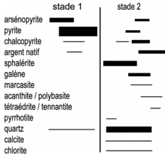
Fig. 2. Succession paragénétique de Zgounder. Paragenetic sequence of Zgounder ore deposit.
