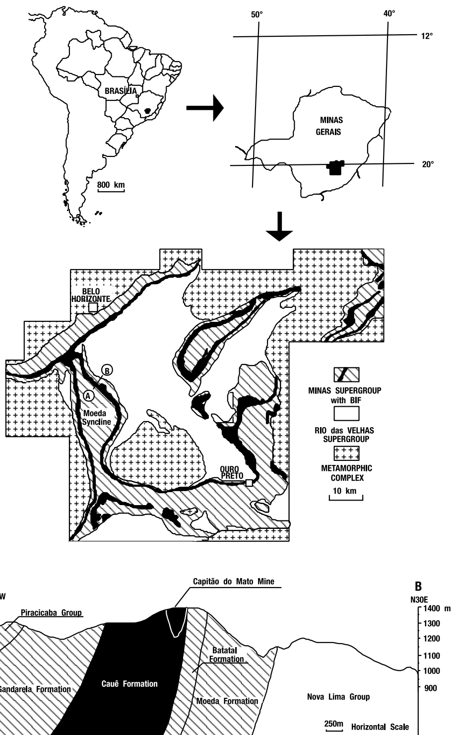
Fig. 1 – Location, geologic map (Marshak and Alkmim, 1989) and geologic section of the Capitão do Mato Mine (geology from Pomerene 1964), Iron Quadrangle, Minas Gerais State, Brazil.
