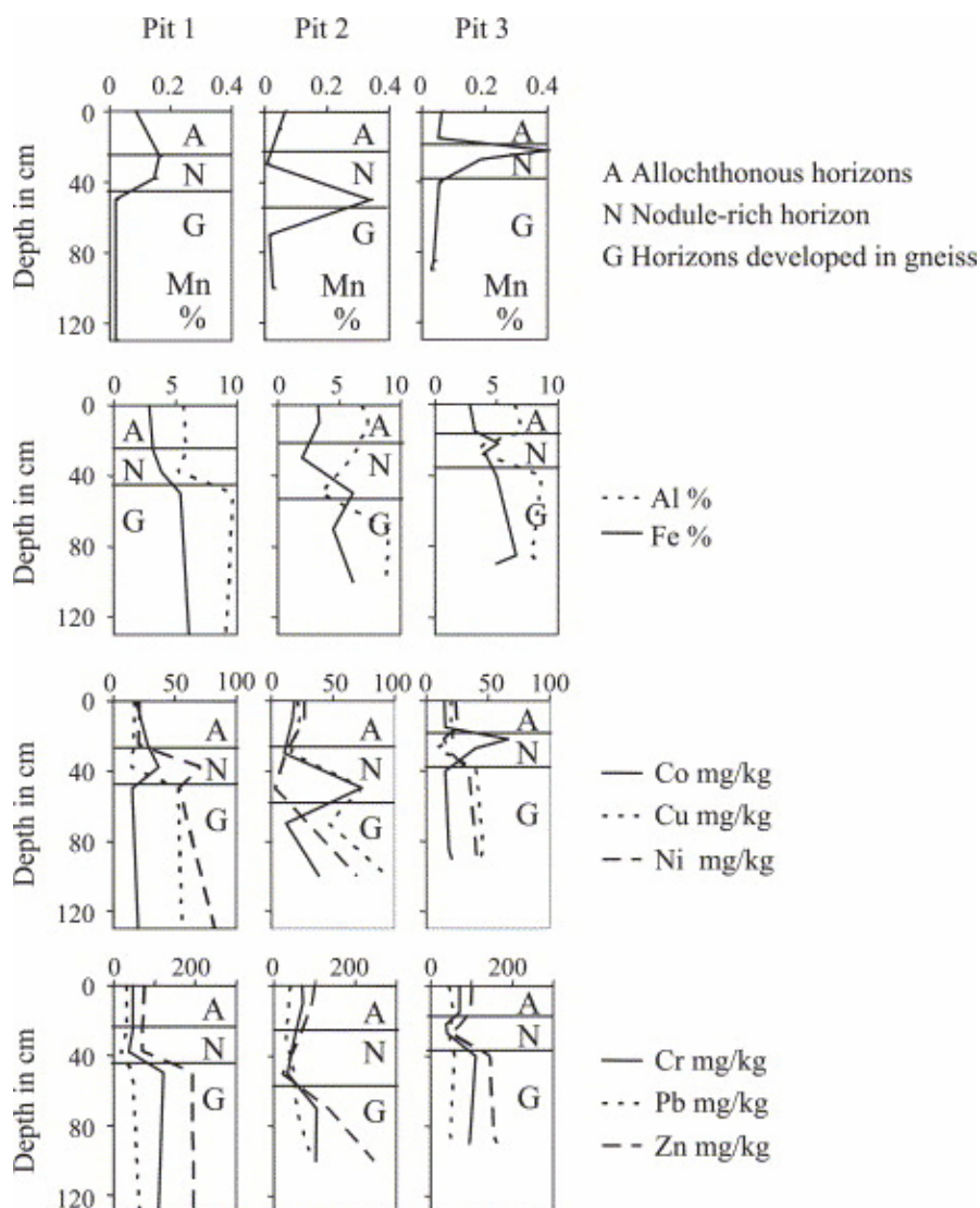
Fig. 3. Chemical profile of the three pits.
