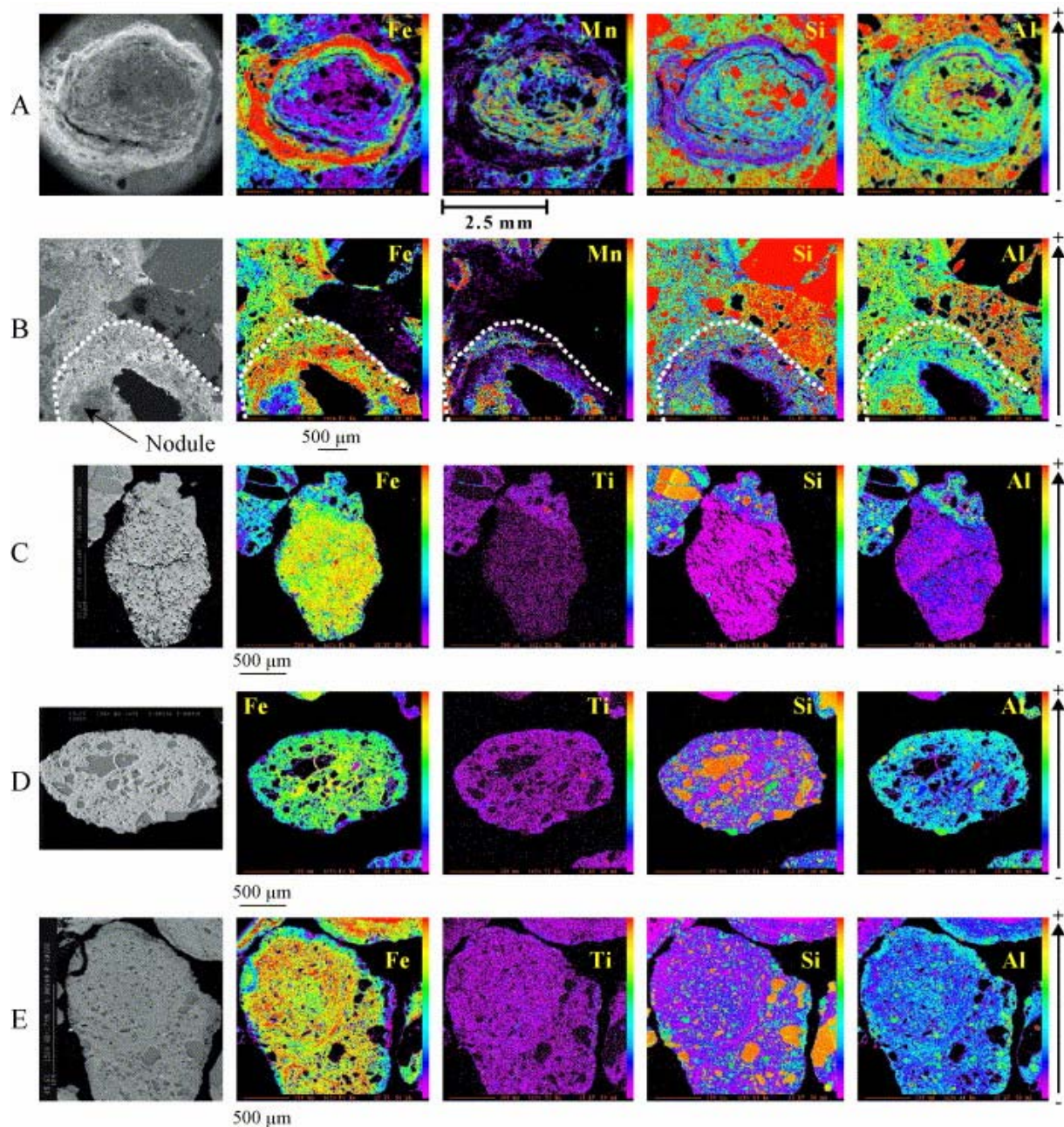
Fig. 2. TE spatial distribution in nodules (electron microprobe mapping). Five nodules are represented (A-E).
