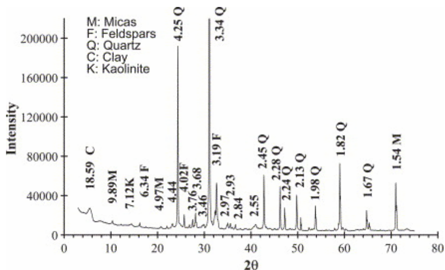
Fig. 4. XRD of the extraction residue of the 1 to 2 mm nodules from pit 2.
