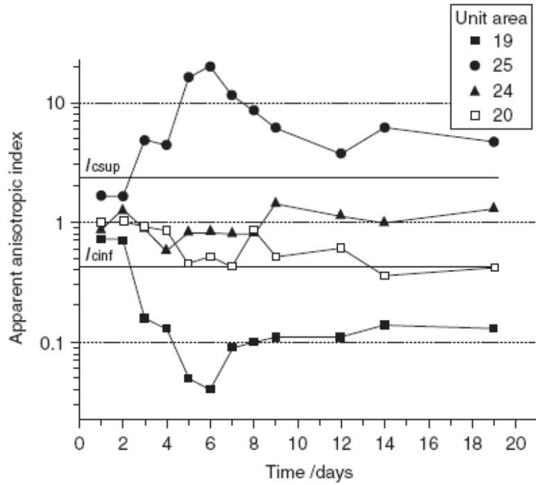
Figure 12 Variation of AAI and comparison with I_{csup} and I_{cinf} thresholds during drying for the four unit areas 19, 25, 24 and 20.
