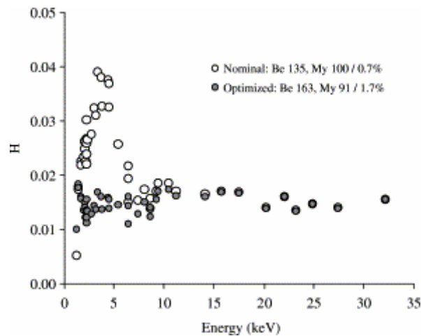
Fig. 3. H values for CERI-CNRS micro-PIXE system using nominal filter parameters and parameter values optimized by the ActiveX component ( Table 1 ).
