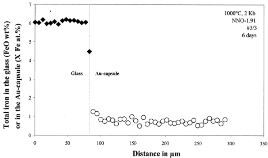
Fig. 8. Evidence of equilibrium attainment between melt and Au-capsule after 6 days-long experiments. Sample #3/3 (see Table 4 and Table 5).
