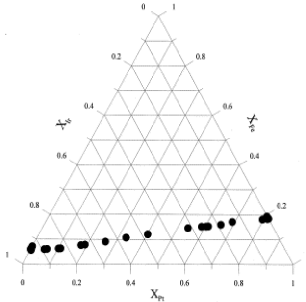
Fig. 9. Non-equilibrated Fe-Ir-Pt alloys and the effect of Pt/Ir on the Fe content of the alloys. The values of a_{\text{FeO}}^{\text{liq}} were calculated from the f_{\text{O}_2} and the composition of Ir-Fe binary (left, a_{\text{FeO}}^{\text{liq}} = 0.081 ) and Pt-Fe binary (right, a_{\text{FeO}}^{\text{liq}} = 0.077 ). See Table 3 and text (5.1.3).
