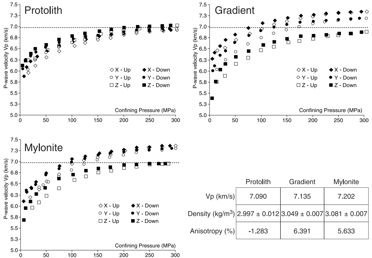
Figure 15. P wave velocity V_p versus confining pressure for three orthogonal directions parallel to the reference axes defined as X the stretching lineation and Z normal to the [XY] mylonite foliation. Horizontal dashed line denotes average V_p of the protolith measured at 300 MPa. Lowest P waves anisotropy A = -1.283\% in the protolith, maximum A = 6.391\% in the gradient zone, and intermediate A = 5.633\% in the mylonite. Fastest P waves are normal to [XY] but near parallel to the protolith foliation, inducing negative calculated anisotropy.
