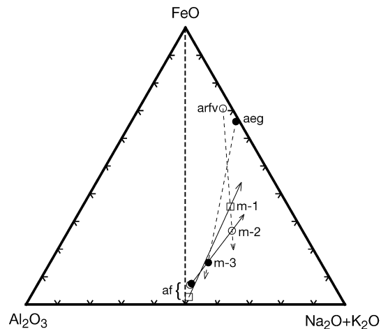
Fig. 10. Positions of selected BL575 and SMN49 melt compositions connected to coexisting minerals by tie-lines in the \text{FeO}^*-\text{Al}_2\text{O}_3-(\text{Na}_2\text{O} + \text{K}_2\text{O}) ternary diagram, illustrating the opposing effects of feldspar, aegirine and alkali amphibole on melt composition. Three topological arrangements are shown: one (□) in which feldspar is the sole Na-bearing crystallizing phase, in which case the melt (m-1) peralkalinity increases continuously; a second case (○) in which the effect of feldspar on melt composition (m-2) is counteracted by the crystallization of an alkali amphibole (arf); a third case (●), corresponding to high f\text{O}_2 conditions, in which the effect of feldspar on melt composition (m-3) is counteracted by the crystallization of aegirine (aeg). The continuous tie-lines represent the effect of feldspar on melt compositions, the dashed tie-lines that of amphibole and clinopyroxene. Phase compositions are from charges 575-24 (□), 49-54 (○) and 49-37 (●).
