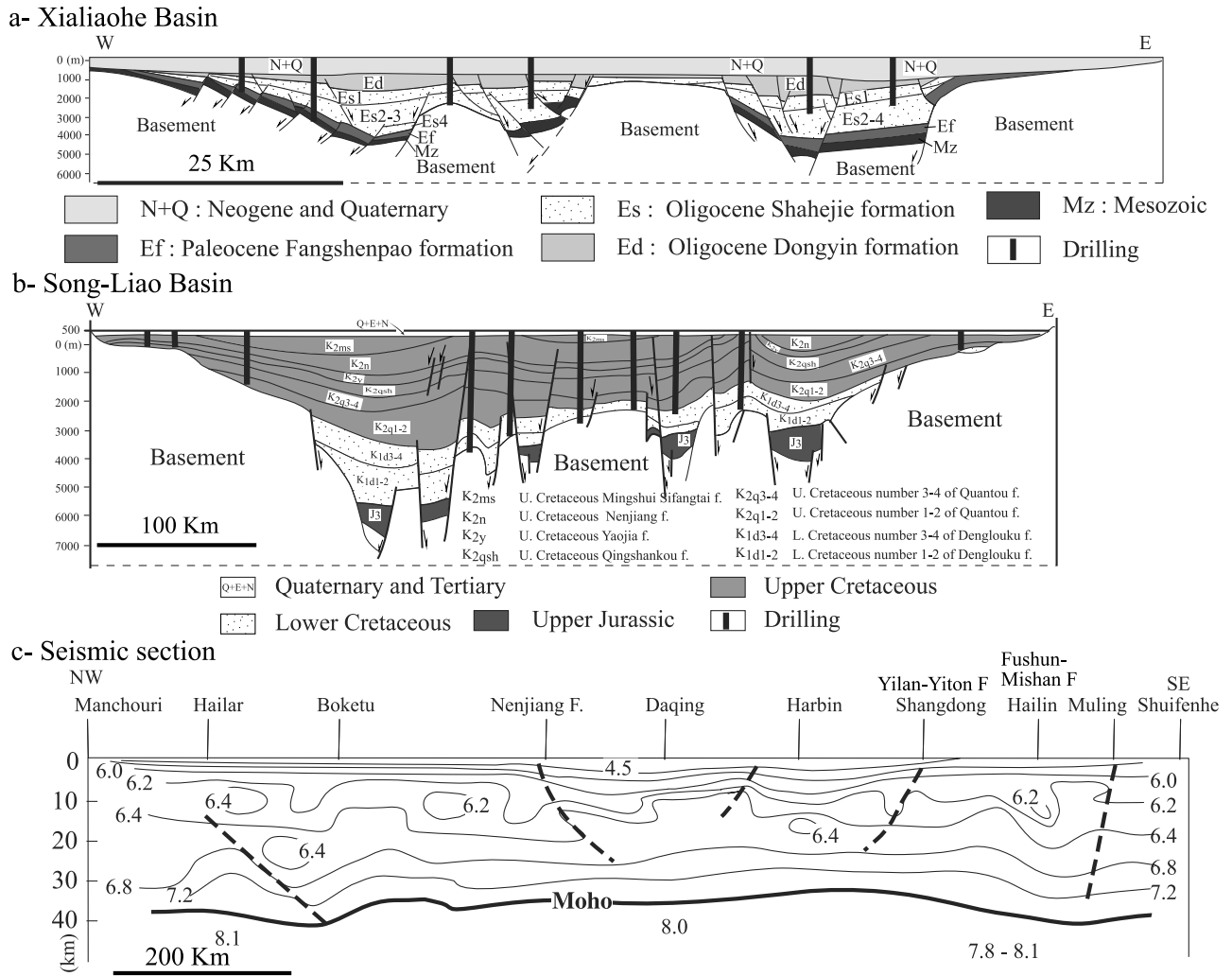
Figure 8. Cross sections through (a) the Xialiaohe basin and (b) the Songliao basin [Chen et al., 1999]. (c) A structural reinterpretation of a seismic section at the crustal scale [after Yu, 1989]. All sections are located in Figure 1.
