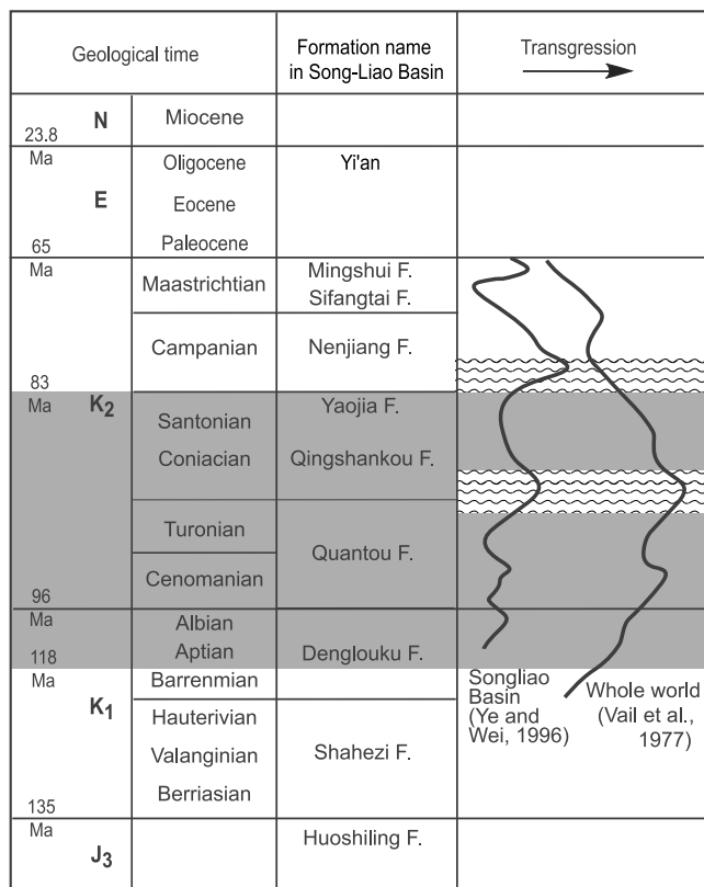
Figure 9. Comparison of the world transgression [after Vail et al., 1977] to that of the Songliao basin [after Ye and Wei, 1996] characterizing the local basin evolution during the Late Cretaceous. The shaded zone presents the possible magnetic remanence age within the Cretaceous Long Normal Superchron (CLNS).
