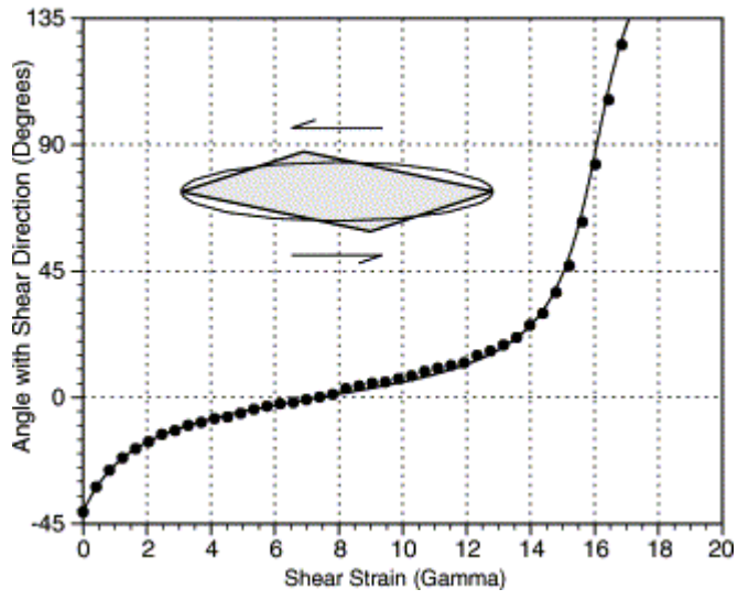
Monoclinic Particle Sinistral Shear Theoretical Curve for Axial Ratio of 5.3
