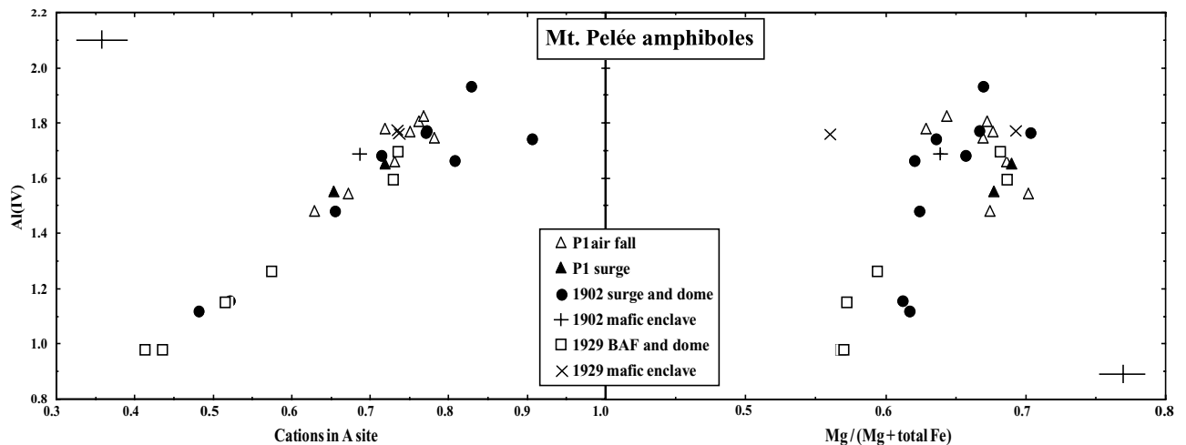
Figure 6. (left) Al(IV) versus number of cations in site A and (right) Mg/(Mg + total Fe) for amphibole phenocrysts from recent eruption products of Mount Pelée. Data for the 1902 and 1929 products are from Gourgaud et al. [1989]. Error bars shown as crosses (top left and bottom right). Amphibole structural formulae calculated on a 23 oxygen basis with all Fe as FeO.
