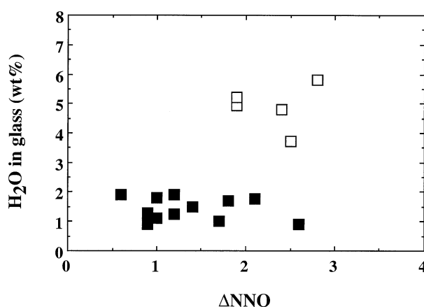
Fig. 4. \text{H}_2\text{O} content of experimental glasses from this study plotted as a function of f\text{O}_2 , expressed as deviation from the NNO buffer ( \Delta\text{NNO} ). (■): experiments performed with the dry starting glass (Table 2); (□): experiments performed with the hydrous starting glass (Table 3).
