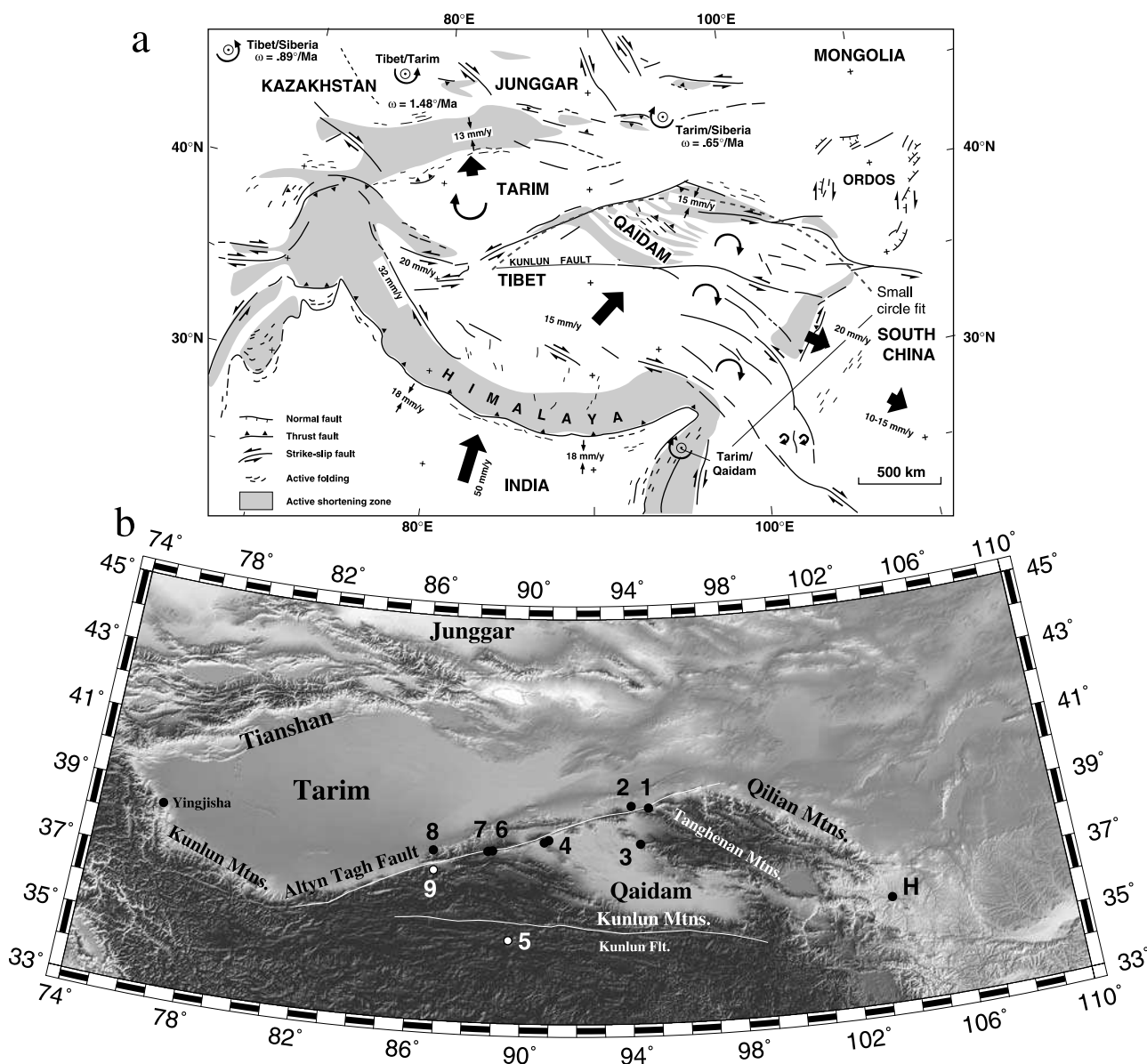
Figure 1. (a) Schematic tectonic map of central Asia [after Avouac and Tapponnier, 1993 ]; (b) Topographic map of sampling areas. Sampling locations from this study: 1, Subei; 2, Aksai; 3, Mahai; 4, Huatugou+Honggouzi+Xorkol; 5, Kekexili; 6, Bulabashi; 7, Valley; 8, Qiemo; 9, Tula. H is the sampling locality of Halim et al. [1998].
