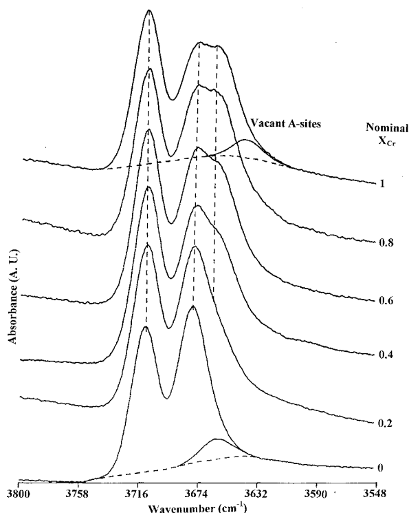
FIGURE 4. Evolution of the FTIR OH-stretching region spectra of pargasite, synthesized at 900 °C and 3 kbar with Cr metal, as a function of nominal X_{Cr} .
