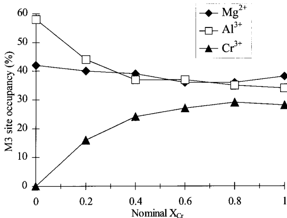
FIGURE 5. Pargasite M3 site occupancy as a function of the nominal X_{Cr} values along the Al-Cr join (900 °C, 3 kbar; experiments with Cr metal).
