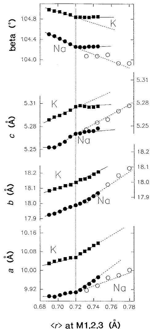
FIGURE 7. Variation in cell parameters of synthetic (nickel, magnesium, cobalt)-richterite, synthetic (nickel, magnesium, cobalt)-potassium-richrichterite, and synthetic (Mg, Fe 2+ )-richterite as a function of the aggregate cation radius at the M1,2,3 sites. The dashed lines show either extrapolations of the linear fit to the (nickel, magnesium)-richterite and (nickel, magnesium)-potassium-richrichterite data or fits to the (magnesium, iron)-richterite data that are constrained to go through the values for end-member richterite.
