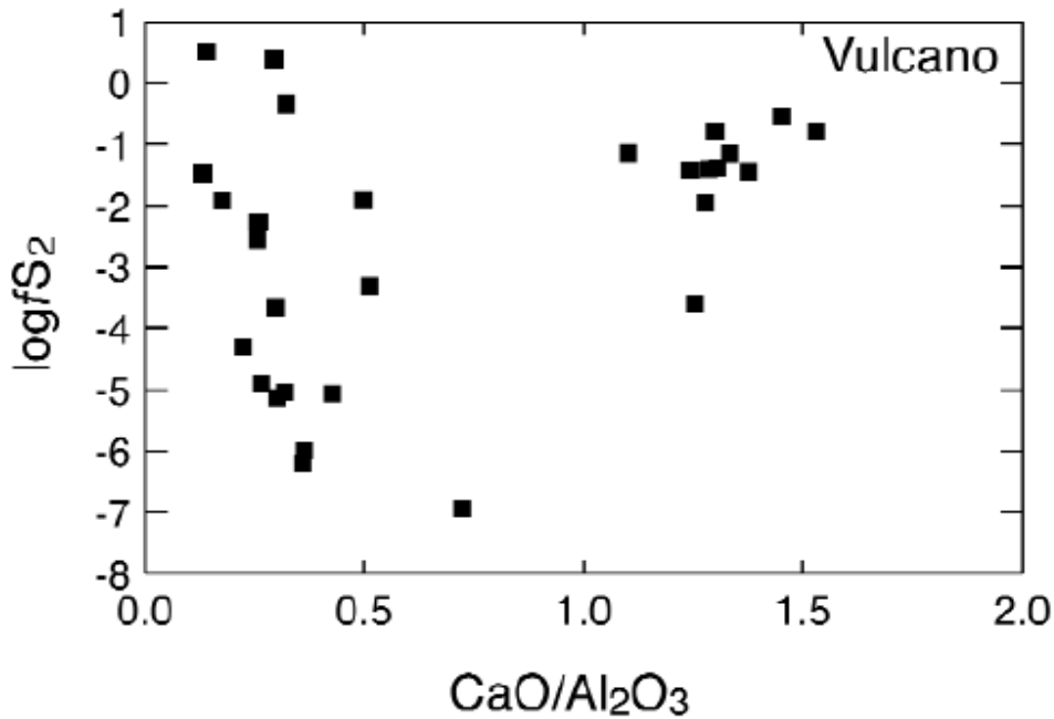
Fig. 6. Evolution of fS_2 with CaO/Al 2 O 3 ratio of Vulcano magmas. The fS_2 is calculated from melt inclusion data (Clocchiatti et al. , 1994a,b; Gioncada et al. , 1998) and eq. (2.1) (see text). Note that the most primitive melts (high CaO/Al 2 O 3 ratio) cluster at around fS_2 of 0.1 bar, whereas the rest of melts defines a negative trend of increasing fS_2 with differentiation.
