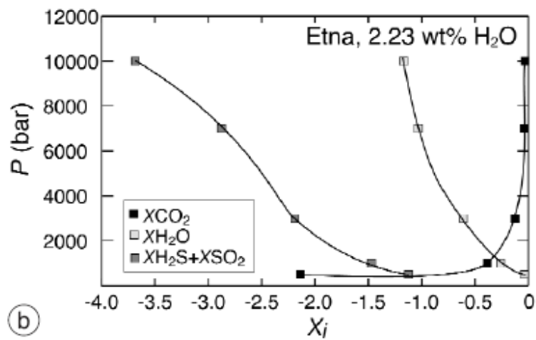
Fig. 14a,b. Evolution of the mole fractions of H 2 O, CO 2 and H 2 S+SO 2 with pressure calculated for melt water contents of 1 (a) and 2.23 (b) wt%, f_{O_2} at NNQ0.35, and melt sulphur contents of 3300-3400 ppm, corresponding to primitive Etnaeian magmas. X_i is the mole fraction of species i .
