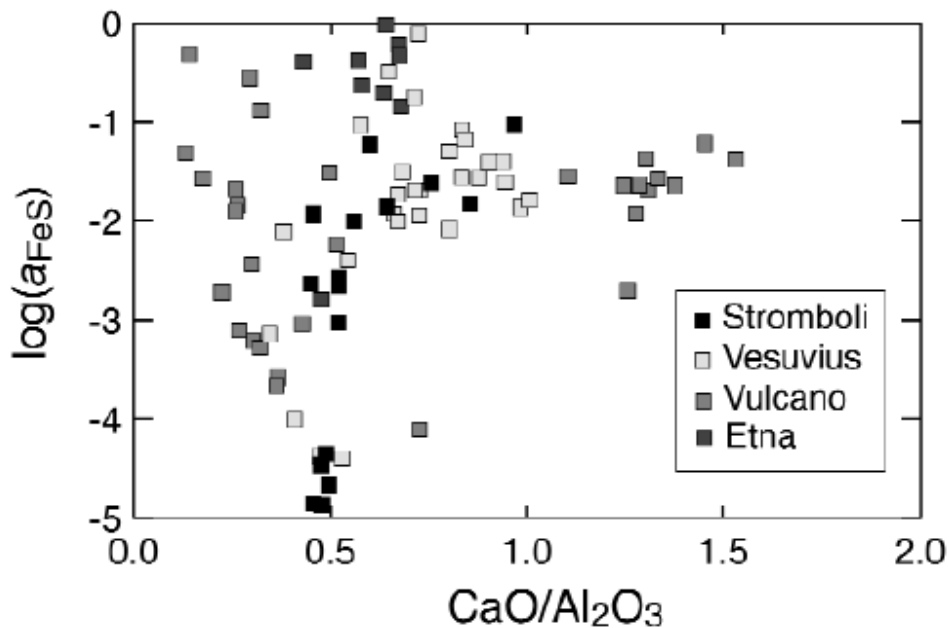
Fig. 4. Calculated activities of liquid FeS plotted versus the CaO/Al 2 O 3 ratio for the four volcanoes considered (see text for explanations). Note that almost all magmas are below saturation conditions with an immiscible sulphide liquid.
