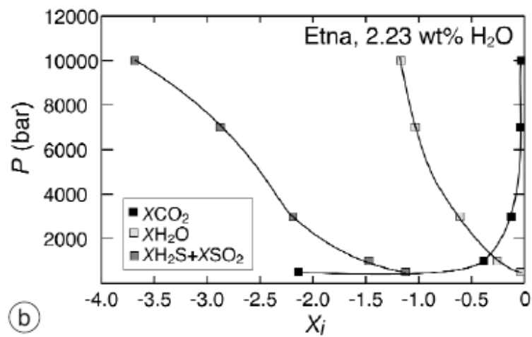
Fig. 14a,b. Evolution of the mole fractions of \text{H}_2\text{O} , \text{CO}_2 and \text{H}_2\text{S}+\text{SO}_2 with pressure calculated for melt water contents of 1 (a) and 2.23 (b) wt%, f_{\text{O}_2} at NNQ0.35, and melt sulphur contents of 3300-3400 ppm, corresponding to primitive Etnaeian magmas. X_i is the mole fraction of species i .
