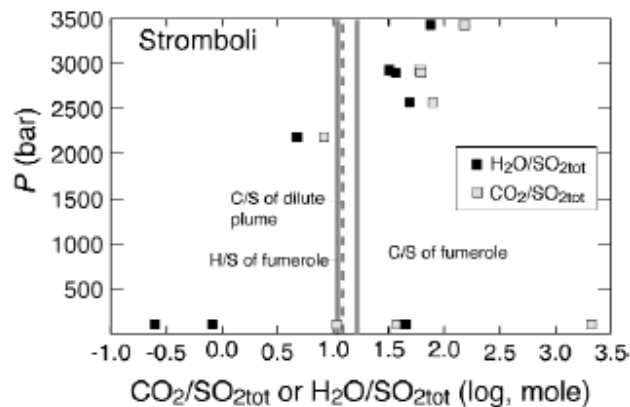
Fig. 9. Pressure evolution of H 2 O/SO 2 tot and CO 2 /SO 2 tot mole ratios of fluids in equilibrium with melt inclusion of Stromboli melt inclusions. The thick grey continuous and dashed lines represent average C/S and H/S ratio measured on a hot fumerole or within the dilute plume at Stromboli (Allard et al. , 1994).
