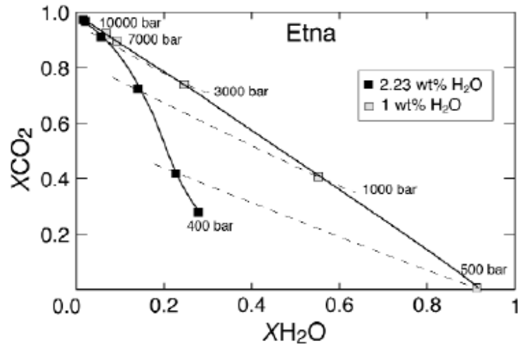
Fig. 15. Evolution of the mole fraction of H 2 O against that of CO 2 calculated for melt water contents of 1 and 2.23 wt%, f_{O_2} at NNO+0.35 , and melt sulphur contents of 3300-3400 ppm, corresponding to primitive Etnaeian magmas. The mole fractions correspond to actual values, that take into account the sulphur species, whose total mole fraction reach values in excess of 0.44 (fig. 14a,b, table II). This is why all the data plot below a mixing line corresponding to a binary H 2 O-CO 2 . Dashed lines represent isobaric conditions calculated for different melt water contents.
