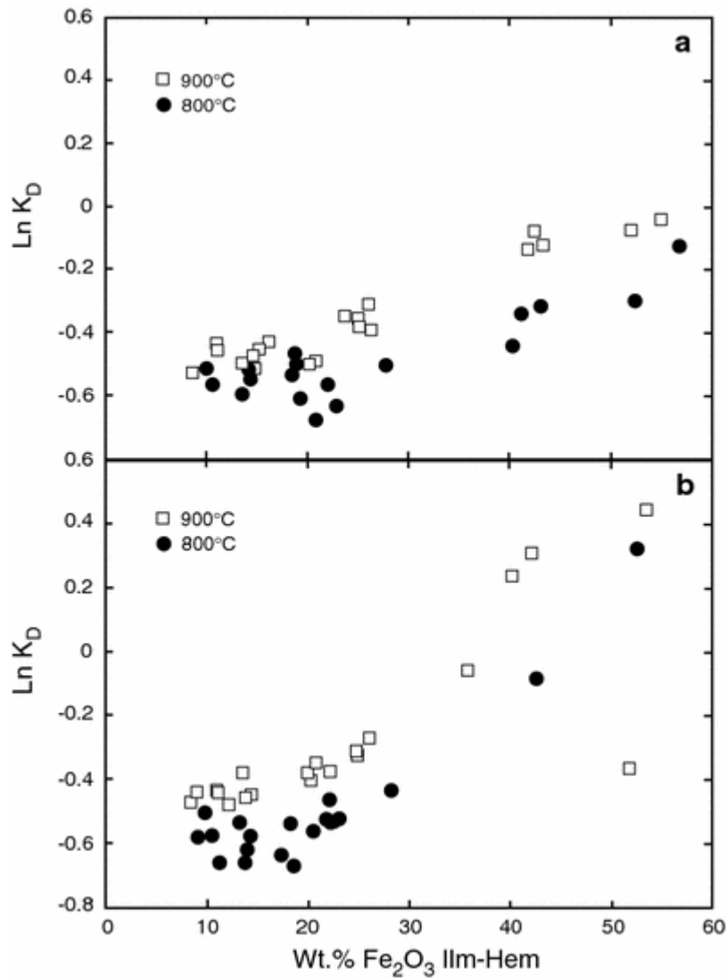
Figure 9 : \ln K_D [K_D = (\text{Mg}/\text{Fe}_{\text{Usp-Mt}})/(\text{Mg}/\text{Fe}_{\text{Ilm-Hem}})] in compositions II and IV (a) and \ln K_D [K_D = (\text{Mn}/\text{Fe}_{\text{Usp-Mt}})/(\text{Mn}/\text{Fe}_{\text{Ilm-Hem}})] in compositions III and IV (b), vs. wt.% \text{Fe}_2\text{O}_3 in Ilm-Hem
