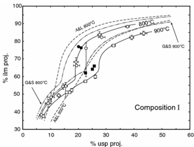
Figure 4 : Roozeboom plot of projected %ilm vs. %usp in experiments on composition I at 800°C (circles) and 900°C (squares). Error bars are \pm 2\sigma or actual range when large and skewed. Continuous lines are hand-drawn fits to our data. Also shown are 800 and 900°C isotherms for the pure system FeTiO from the formulations of Andersen and Lindsley (1988) and Ghiorso and Sack (1991). Two experiments (800 and 890°C) on the HAMQ buffer are shown by filled circles and filled squares, respectively
