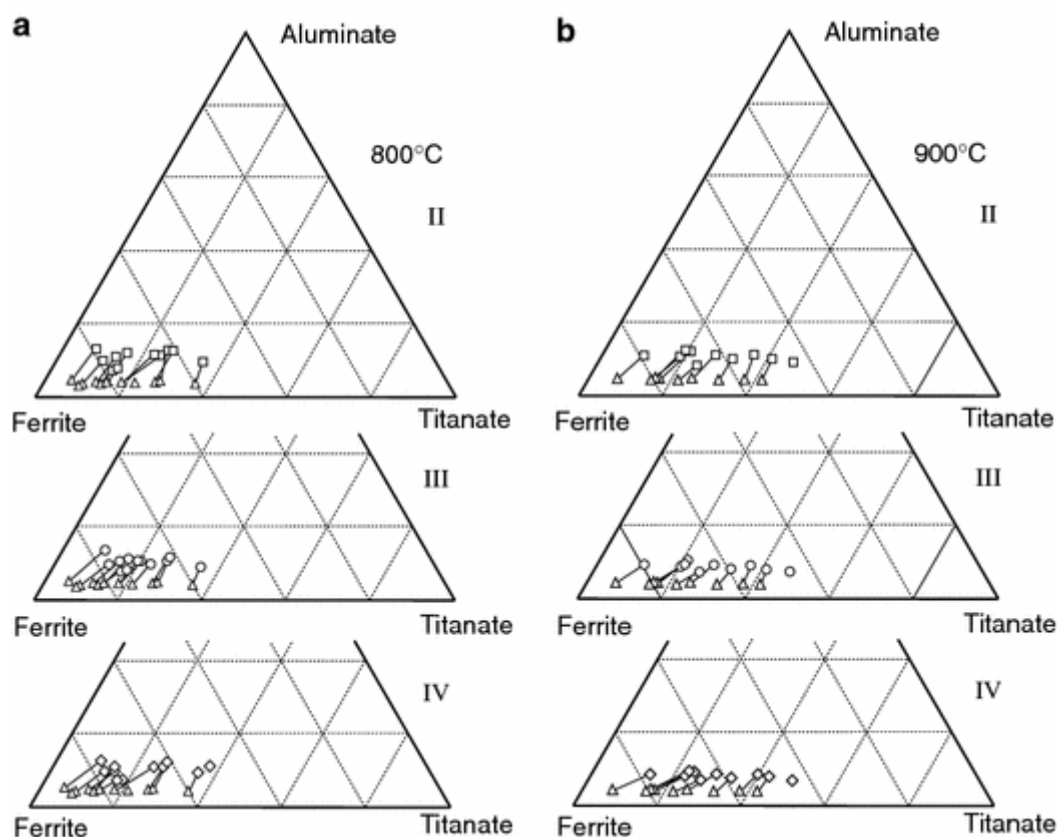
Figure 5 The composition of FeTi-spinels at 800°C (a) and 900°C (b) in the ternary diagram ferrite–titanate–aluminates. Triangles are composition I spinels, squares composition II, circles composition III, and diamonds composition IV. Tielines link products of the same experiment; they are not coexisting pairs
