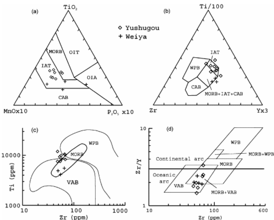
Fig. 7. Discrimination diagrams of tectonic settings for the Weiya and the Yushugou mafic granulites (a) TiO_2 – MnO – P_2O_5 diagram (after Mullen, 1983); (b) Ti – Zr – Y diagram (after Pearce and Cann, 1973); (c) Ti – Zr variation plot (after Pearce, 1982); (d) Zr/Y – Zr plot (after Pearce and Norry, 1979). MORB, Middle ocean ridge basalt; OIT, Ocean island tholeiite or seamount tholeiite; OIA, Ocean island alkali basalt or seamount alkali basalt; IAT, Island arc tholeiite; CAB, Calc-alkaline basalt; WPB, Within-plate basalt; VAB, Volcanic arc basalt.
