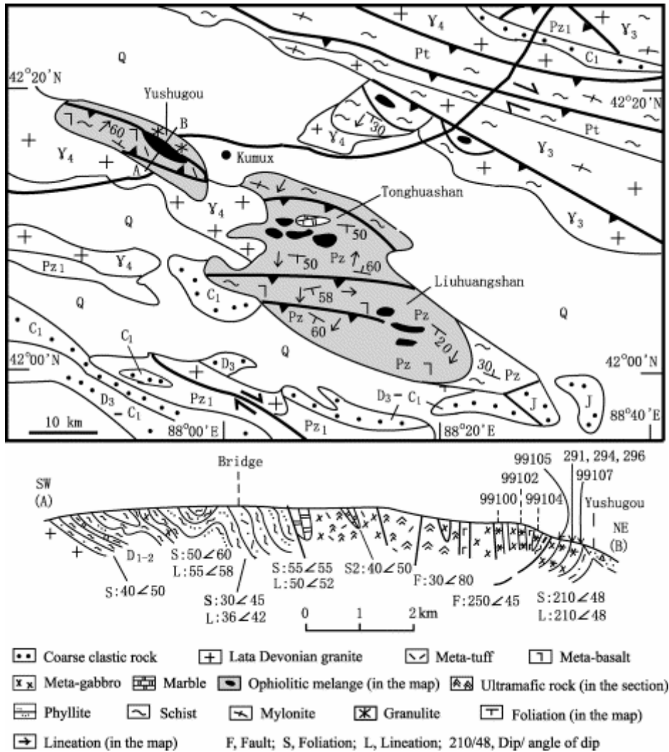
Fig. 3. Simplified geological map (upper) and structural section (lower) for the Yushugou granulate (modified from 1:1000000 Xinjiang geological map, XBGRM, 1992)
