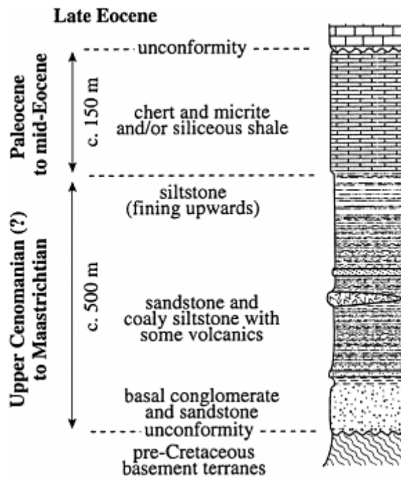
Fig. 3. Sketch columnar section of the Late Cretaceous to mid-Eocene sedimentary megasequence of New Caledonia (Noumea region) showing the late Cretaceous fining upwards clastic sequence and the Paleocene to mid Eocene siliceous and carbonated post-rift sequence.
