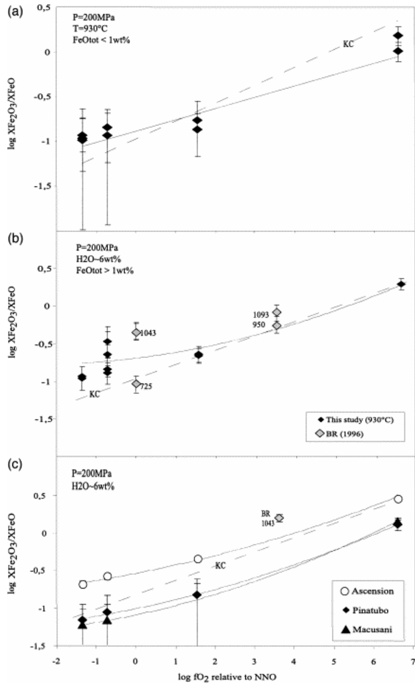
Fig. 4. Plot of \log(X_{Fe_2O_3}/X_{FeO}) against \log fO_2 for synthetic metaluminous compositions (a: FeO_{tot} concentrations <1 wt.%; b: FeO_{tot} concentrations >1 wt.%) and Ascension, Macusani and Pinatubo compositions (c) at 930°C, 200 MPa, H_2O -saturated. Data in Table 5. Dashed lines labelled KC show X_{Fe_2O_3}/X_{FeO} ratios calculated after Kress and Carmichael (1991) for the synthetic metaluminous compositions (a, b) and Ascension composition (c). Solid curves are polynomial fits to the data points. Data of Baker and Rutherford (1996) plotted as BR (96) with temperature indicated in degrees Celsius. Abbreviations and notations as in Fig. 2. Note the non-linear relation between experimental ferric–ferrous ratios and fO_2 , and the oxidizing effect of water <NNO+1 (see text).
