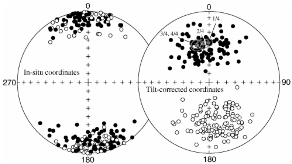
Figure 4. Stereonet plot of 222 magnetization directions used to constrain the magnetostratigraphy shown in Figure 5. Open (solid) circles are projected on the upper (lower) hemisphere. Stars and 95% confidence ellipses are mean values of each quarter of the section (1/4 is top; 4/4 is bottom) (data from Table 1).
