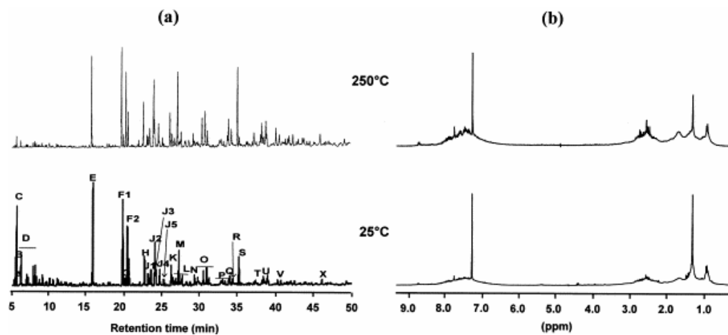
Fig. 9. (a) Gas chromatograms and (b) ^1\text{H-NMR} spectra of the soluble fractions from the raw perhydrous coal and its pyrolysate at 250^\circ\text{C} .
