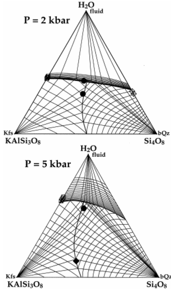
Fig. 6. Calculated isotherms on the liquidus surface in the system \text{KAlSi}_3\text{O}_8 – \text{Si}_4\text{O}_8 – \text{H}_2\text{O} at 2 and 5 kbars, 700°C to 1700°C with 50°C increments. Solid symbols denote measured compositions of minimum melting at \text{H}_2\text{O} -saturated and -undersaturated conditions from Pichavant et al. (1992); 720°C, 750°C, 835°C, circles and Becker et al. (1998); 1030±10°C, diamond. Open diamonds are measured \text{H}_2\text{O} solubility at 1200°C and 1300°C (Holtz et al., 2000). Squares are solubility data at 1000°C, 2 kbars and 900°C to 1200°C, 5 kbars from Behrens et al. (2000).
