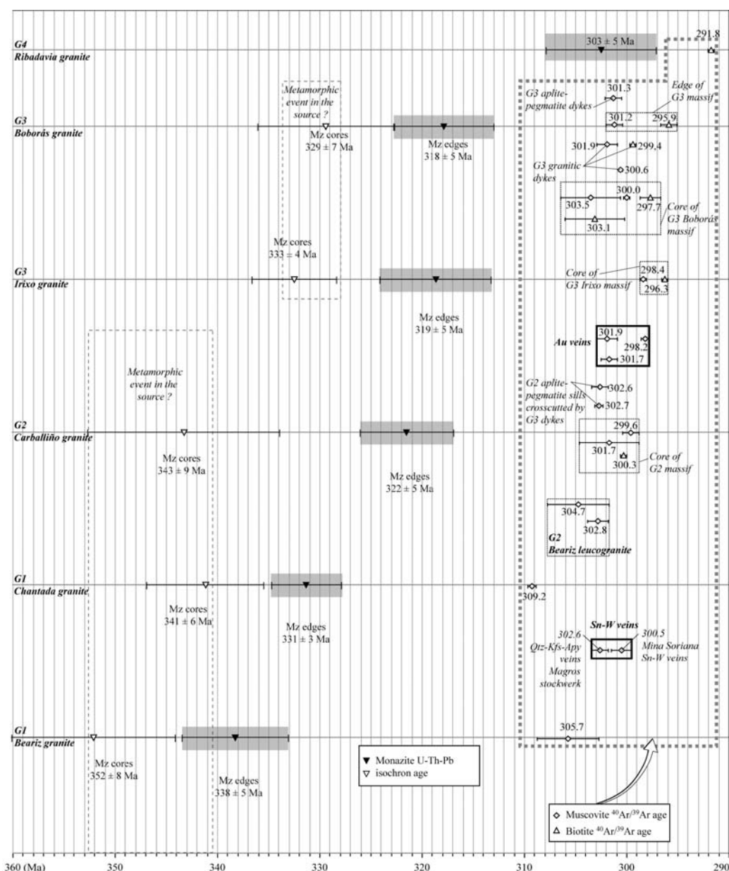
Fig. 3. Synthesis of the ages obtained by ^{40}\text{Ar}/^{39}\text{Ar} method on granites and mineralization and EPMA ages on monazite (U-Th-Pb isochron ages) on granites. Granites emplacement ages are given by ages of monazites edges, metamorphic event in the sources of granites are given by ages of monazites cores.
