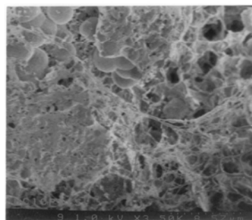
Fractured surface of a phosphatic pellet, apatite dissolved by HCl, observed under SEM, and showing intrapelletal organic matter
