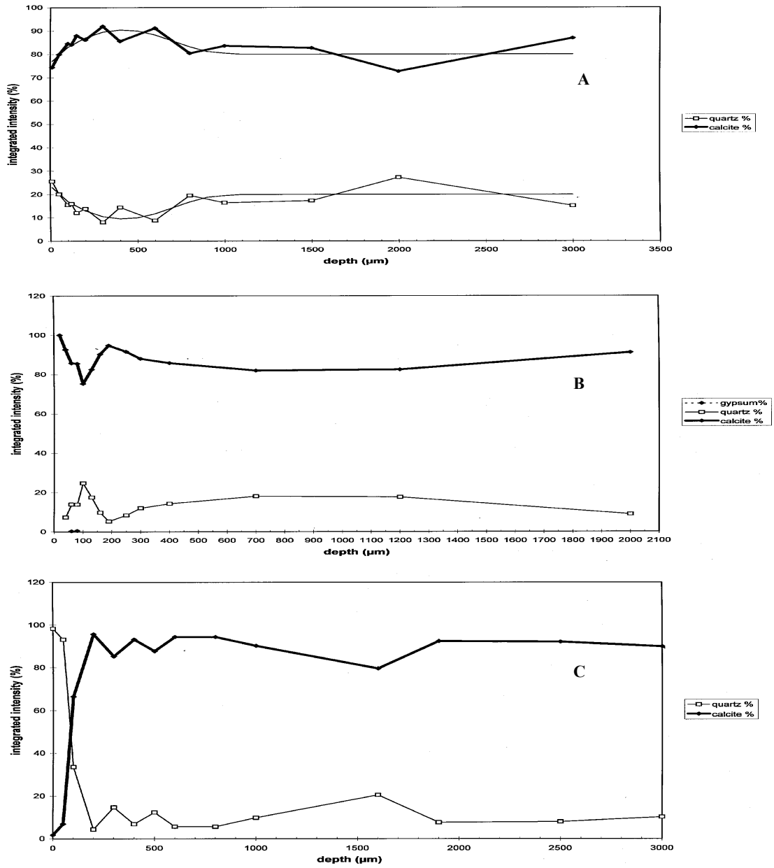
Figure 4. Mineralogical evolution for different depths from the patina A: outside column sample (OC) B: inside lintel sample (IL) C: buried shell sample (BS)
