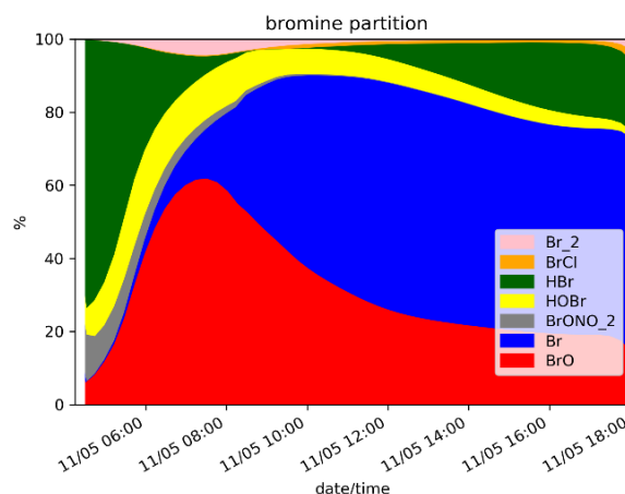
670 Figure 8: Similar to Fig. 3 but the simulation D.Emis.NO.
