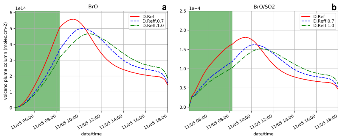
695 Figure 9: Similar to Fig. 4a and 4f but the simulations testing the sensitivity to the effective radius of sulphate aerosols: D.Ref, D.Reff.0.7 and D.Reff.1.0.
