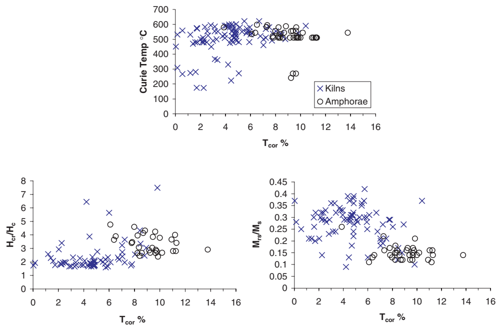
Figure 8. Rock magnetic parameters Curie temperature, the ratio of coercivity of remanence to coercivity H_{cr}/H_c and the ratio of the remanent saturation magnetisation to the saturation magnetisation M_{rs}/M_s plotted against the cooling rate correction T_{cor} .
