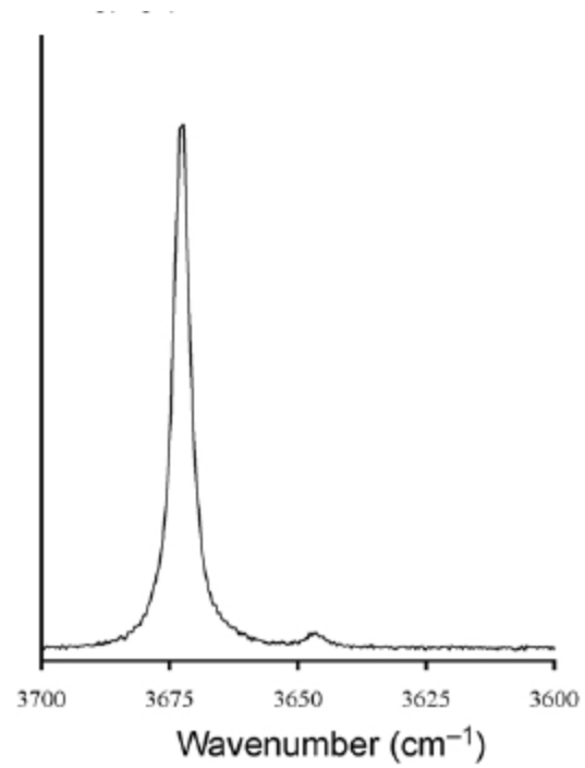
Figure 10: Raman spectra of VAN pyrophyllite sample in the OH stretching zone.
