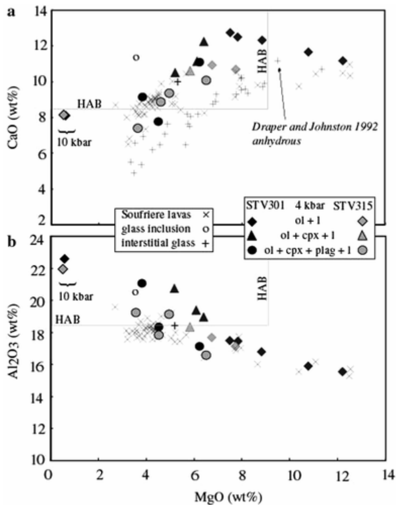
Fig. 5 MgO variation diagrams (a CaO; b \text{Al}_2\text{O}_3 ) for experimental glasses (this study) and Soufriere natural products (Fig. 4). Experimental data at 4 kbar except otherwise stated (10 kbar). Data points separated by phase assemblage, with starting glasses and ol + l charges plotted under the same symbol. For STV315, all cpx + plag-
