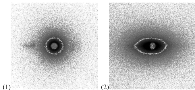
Figure 2 Two-dimensional SAXS images recorded in the two configurations (1) and (2) (see Fig. 1). In both images, a narrow range of intensities has been painted white so as to highlight the shape of an iso-intensity line: in (1), the image is isotropic; in (2), it is strongly anisotropic.
