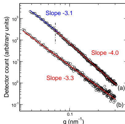
Figure 3 Radial intensity profiles from a SAXS image recorded at 393 K: (a) along the ellipse's long principal axis (close to horizontal in Fig. 2(2)), and (b) along the ellipse's short principal axis (close to vertical in Fig. 2(2)).
