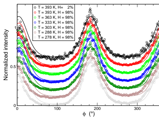
Figure 4 Azimuthal intensity profiles for a series of SAXS images recorded at decreasing temperature values. Maier-Saupe fits are superimposed to the data; they provide the ODP function for the nematic order of scattering objects in the sample.
