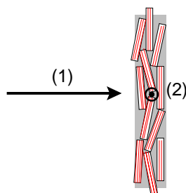
Figure 1 Sketch of a vertical cut of one 2 \times 2 \times 6 \text{ mm}^3 dry-pressed Na-fluorohectorite sample, as it stands in the beam. The gray shadings denote the sample's mesopores, while the red lines represent the nano-porosity inside the nano-stacks. Two configurations were used: one in which the beam is oriented with respect to the sample according to the direction denoted (1), and one in which it is oriented according to the direction denoted (2).
