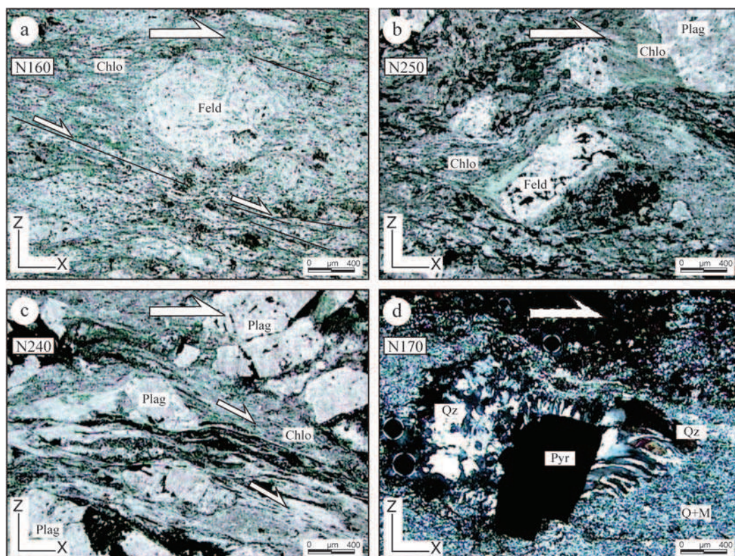
Figure 7 Photomicrographs showing examples of north-verging deformation in the Ordovician volcanics and Mishigou mélangé, Mishigou area. a: Chloritized feldspar porphyroblast in a graywacke, top-to-the-N340 shearing, PPL; b: Feldspar clast with chlorite asymmetric pressure shadows in an andesitic tuff, top-to-the-N70 shearing, PPL; c: Shear-bands with chlorite and oxides in a tuff, top-to-the-N60 shearing, PPL; d: Quartz fringes around a pyrite grain in a micro-sandstone, top-to-the-N350 deformation, CPL. Feld.: feldspar; Chlo: chlorite; Qz: quartz; Oxi: oxides; Plag: plagioclase; Pyr: pyrite; Q+M: quartz-mica matrix.
