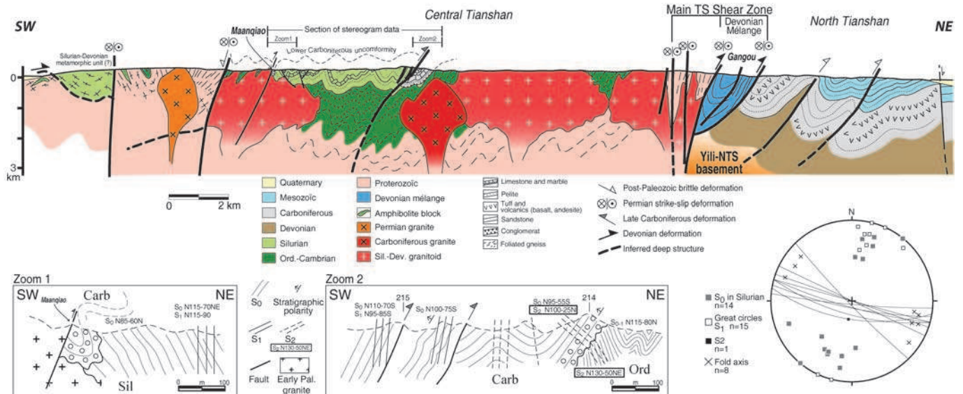
Figure 4 Synthetic cross-section of Central and North Tianshan along the Kumux-Toksun transect, and detailed structural data of some segments.
