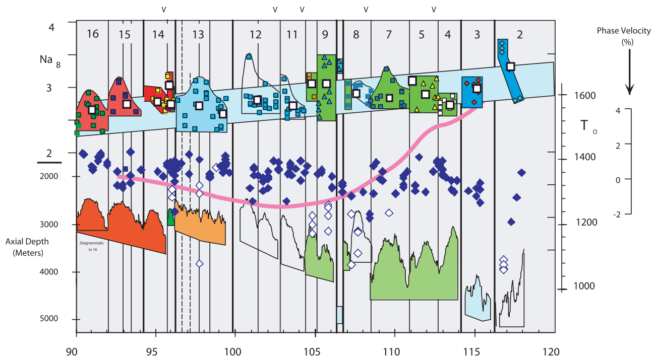
Figure 4. Profiles along the SEIR between 90°E and 118°E, showing, from top to bottom, \text{Na}_8 concentration calculated using the equation of Klein and Langmuir [1987]. Open squares are segment averages, smaller segments are values for individual glass groups. Smaller fields encompass the range of values for each segment. Linear background fields indicate range predicted from the global correlation of Klein and Langmuir [1987]. T_0 is the temperature of initial melting [ Niu and Batiza , 1991]. Solid diamonds are normal MORBs; open diamonds are enriched MORBs. Curve behind data represents variations in Rayleigh waves phase velocity anomaly (in %) at T = 200 s [ Roult et al. , 1994]. Axial depth is shown by the lower group of irregular fields. Shaded fields indicate intrasegment morphological transitions. Vertical lines represent segment boundaries. After Christie et al. [1995].
