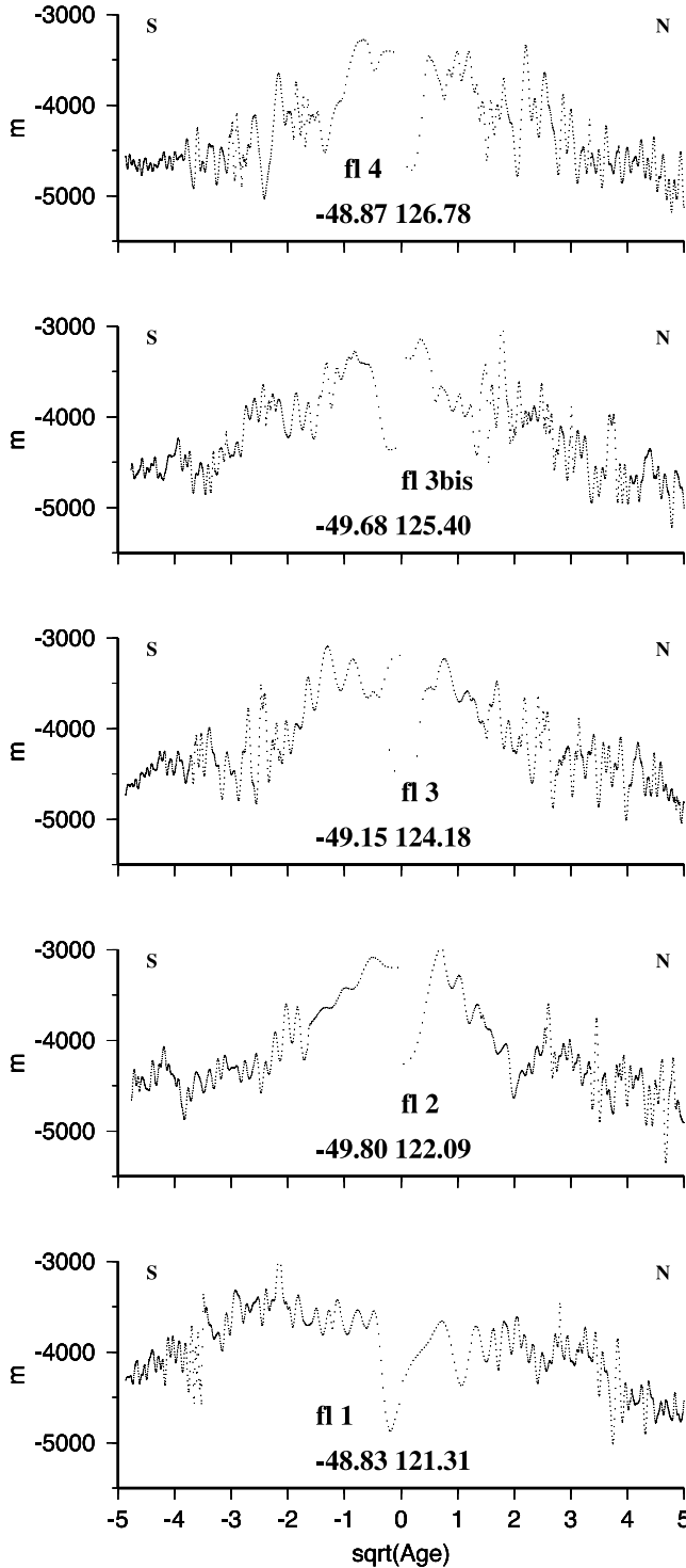
Figure 8b. Basement depth plotted versus the square root of crustal age along selected flow lines crossing the SEIR between 120°E and 128°E (see location in Figure 2) based on the kinematic parameters (poles and rotation angles) of Marks et al. [1999]. Zero-age coordinate is indicated for every flow line. Flow line numbers refer to those indicated in Figures 2 and 5. Note that the subsidence averages (see text) between 120°E and 128°E have been computed without flow line 1.
