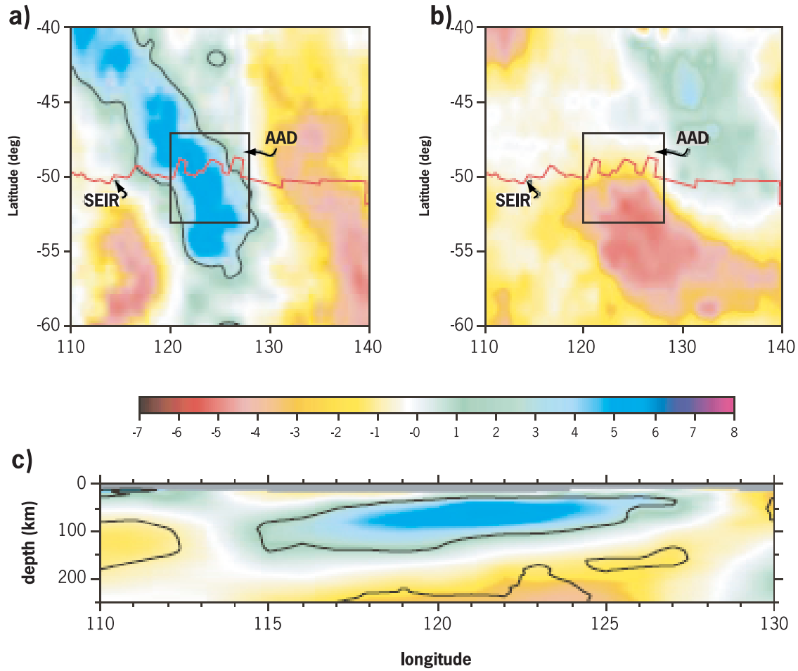
Figure 3. Images of the Australian-Antarctic Mantle Anomaly (AAMA). (a) Horizontal slice of the Vs model at 60 km depth plotted with respect to an age-dependent model. Black contours indicate +3% perturbations. (b) Similar to Figure 3a, but at 200 km depth. (c) Along-strike vertical slice. After Ritzwoller et al. [2003].
