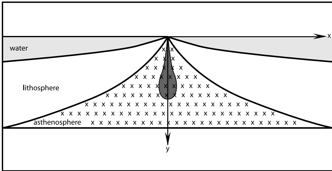
Figure 12. Sketch explaining the signification of parameter \phi_m : an “homogeneous melt fraction,” which would be equally distributed within the asthenosphere (crossed area). This parameter is supposed to depend on the mantle temperature, T_m , at the base of the plate. This parameter \phi_m must not be mistaken with the partial melt fraction (a function of P and T ) that characterizes the zone below the ridge from which melt is extracted to produce the axial crust (grey area).
