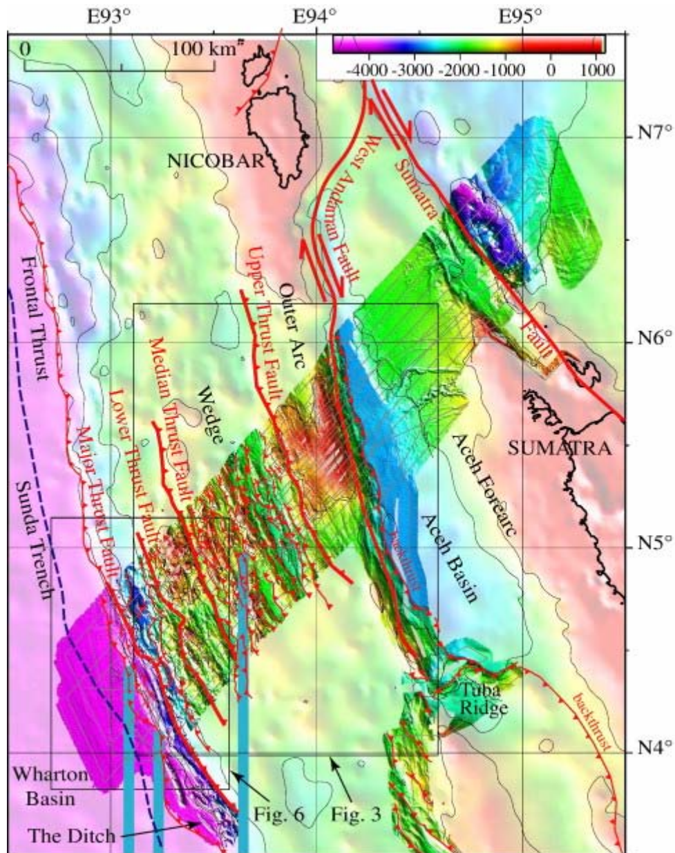
Figure 2: Swath-bathymetric data collected along a 370x75 km stripe located southeast of the India-Indonesia water limit over the regional bathymetry [20]. Light from the southwest. The thin gray lines are tracklines along which swath bathymetric and 3.5 kHz data were continuously collected. Main structural elements in red. Lines with triangles are thrust faults. Thick continuous red lines with triangles are main thrust faults determined from swath-bathymetric and 3.5 kHz data. The solid N-S trending blue lines are the locations of N-S fracture zones of the Wharton Basin and their associated N-S trending valleys in the wedge.
