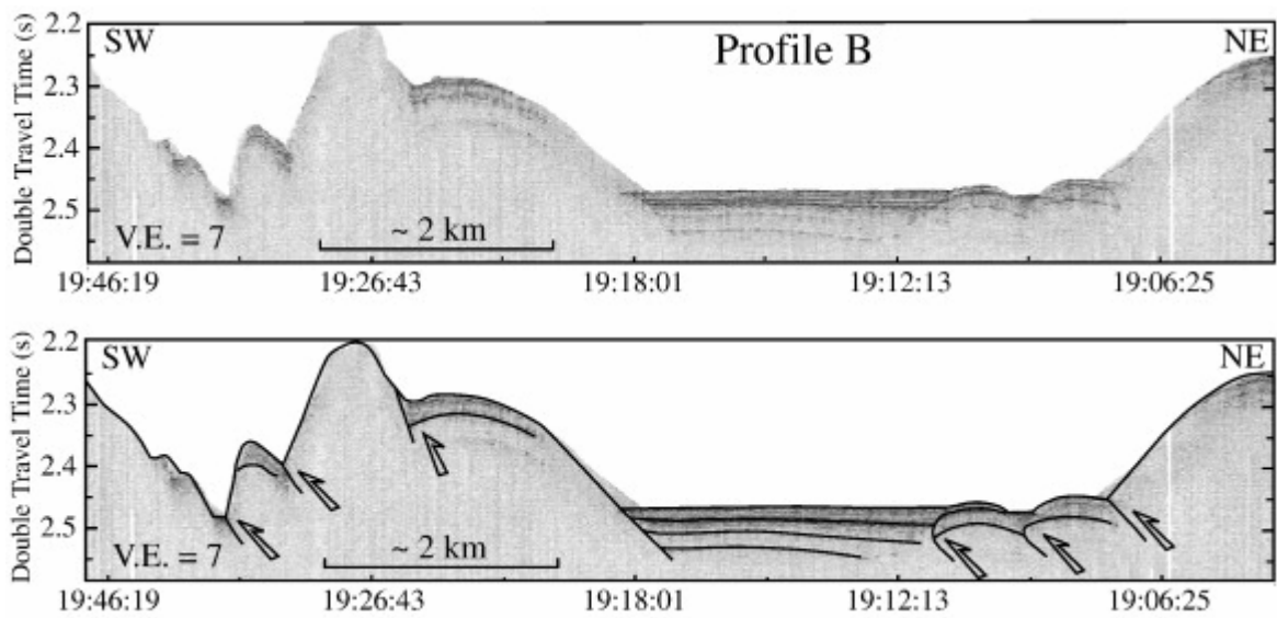
Figure 5: 3.5 kHz Profile B located in Fig. 3 across the same piggy-back basin than in Fig. 4, with numerous seaward vergence thrust faults showing signs of recent tectonic activity.
