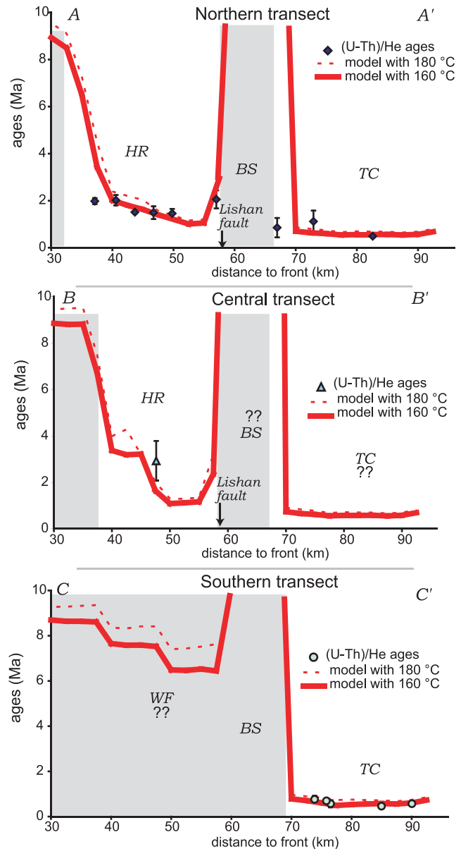
Figure 10. (U-Th)/He ages on detrital zircon [Beyssac et al., 2007] with 2- \sigma error bars and predictions from our thermokinematic model by assuming a closure temperature of 180°C (dashed red line) and 160°C (solid red line). Shaded areas indicate where the ages are partially reset or nonreset. In the case of the central transect, no data are available for the BS and TC, and we assume that the extent of the area where ages are not reset is similar to that of the northern transect. Also data are not available over the WF of the southern transect, and we suppose that ages may be not reset or only partially reset. The predicted peak metamorphic temperatures (Figure 8) over the WF along the southern transect suggest possibly reset ages, but there are no data to test this prediction.
