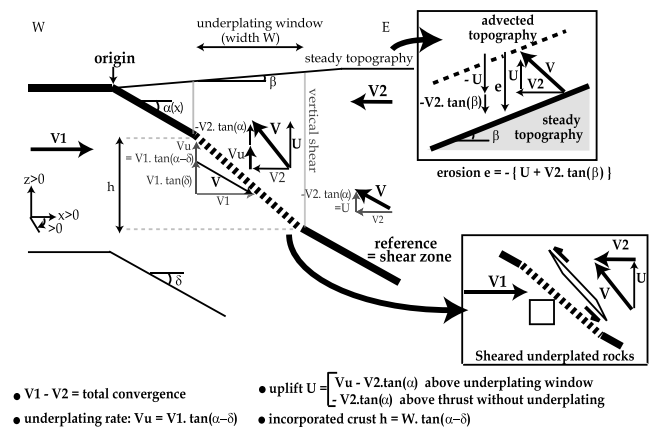
Figure 6. Geometry and kinematics in our thermokinematic finite element model. The basal shear zone of the orogen is taken as the reference for the velocity field. The topography is assumed steady state (constant in this reference frame). The divergence of the velocity field is zero to insure mass conservation. Deformation of the wedge, required to accommodate lateral variations of the underplating rate, is restricted to hinge lines assumed vertical (vertical gray lines). For simplicity, the footwall is assumed undeformed once it has passed through the hinge line at x = 0 . This is not necessarily true in reality but a reasonable assumption given that the data analyzed here are not sensitive to any eventual footwall deformation. Where the shear zone and the Moho are parallel ( \alpha = \delta ), underplating is not allowed. The thickness h of the crust incorporated into the orogen may be easily calculated from the dip angles \alpha and \delta of the shear zone and of the underthrusting velocity, as well as from the width W of the underplating window. Since topography is assumed to be steady state, modeled erosion e has to balance the total rock uplift U as well as the lateral advection V_2 of the topography (top inset). Given the velocity field, underplated units are deformed and sheared across the basal decollement, and the shear direction is parallel to the decollement. This is illustrated in the bottom inset by the deformed geometry acquired across the underplating window of an initially square volume. See text for further details.
