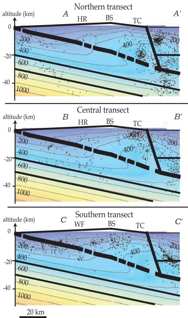
Figure 14. Predicted thermal structures for the three transects investigated in this study. Isotherms are represented by 100°C contours. Also shown is relocated seismicity from Wu et al. [2007], retrieved along a 30 km wide swath centered along each one of the three transects located in Figure 1. Only the seismicity prior to the Chi-Chi earthquake from 1991 to September 1999 is plotted. The correlation of seismicity with topography and with the thermal structure, as noticed in earlier studies [e.g., Lin , 1998], holds to first order: a seismic gap seems to coincide with the high topography (except for the southern transect), and with the 350°–400°C isotherms (except for the northern transect along the suture zone).
