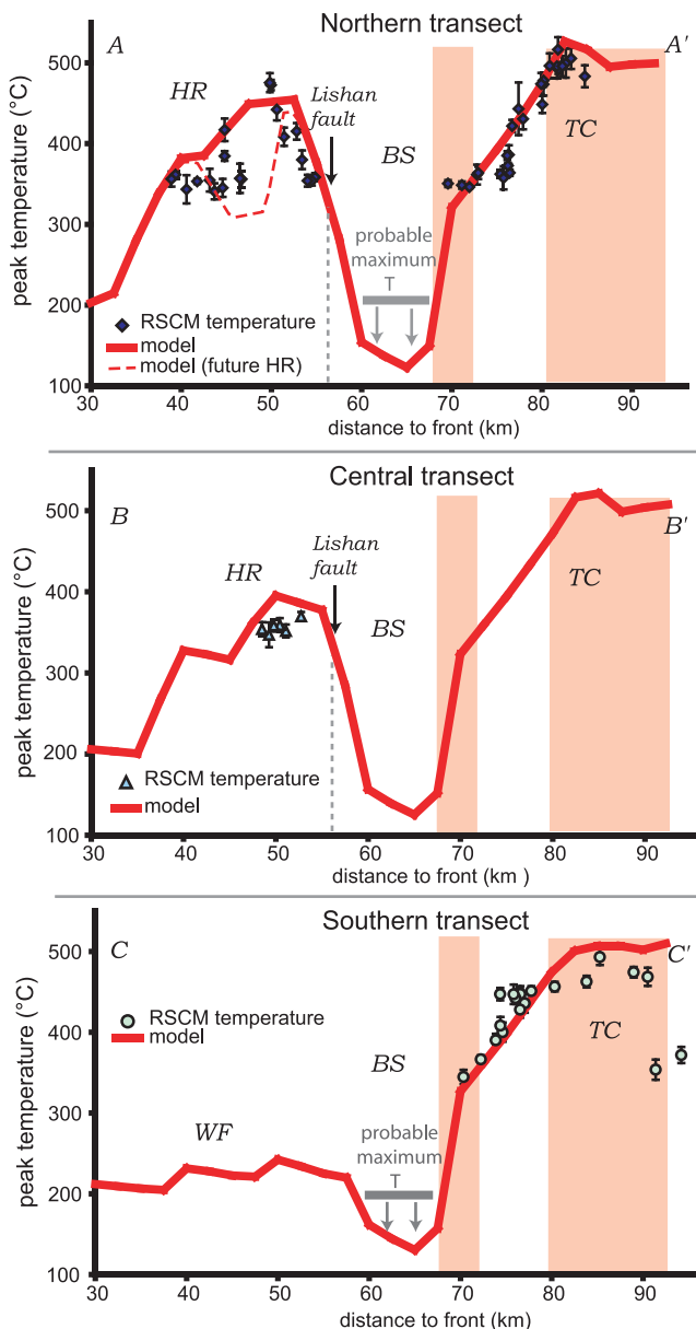
Figure 8. Peak metamorphic temperatures measured from RSCM thermometry [Beyssac et al. , 2007] and predicted by our thermokinematic model (red line) for the northern, central, and southern transects (Figure 1). Error bars represent a 2\text{-}\sigma interval. A probable maximum temperature of 200^\circ\text{C} is given over most of the BS for the northern and southern transects because most thermochronological ages are not reset (Figures 9 and 10) in this region. It is possible that this is also the case for the central transect, for which data are not available over the BS and TC. Shaded areas indicate where the model predicts peak metamorphic temperatures that were reached in the model during accretion to the wedge: this is the case for the high RSCM temperatures of \sim 500^\circ\text{C} over the eastern TC, and for the temperatures of \sim 350^\circ\text{C} over the eastern BS units (Pilushan formation). Our model therefore suggests that most of the observed peak temperatures characterize the thermal structure of the passive margin (nonshaded regions). The dashed red line over the HR in the case of the northern transect indicates the pattern predicted for an additional 0.5 Ma long period of underplating below this region. In this case, underplated rocks are exhumed at the surface and show lower peak temperatures of \sim 300^\circ\text{C} that are acquired during accretion to the orogen.
