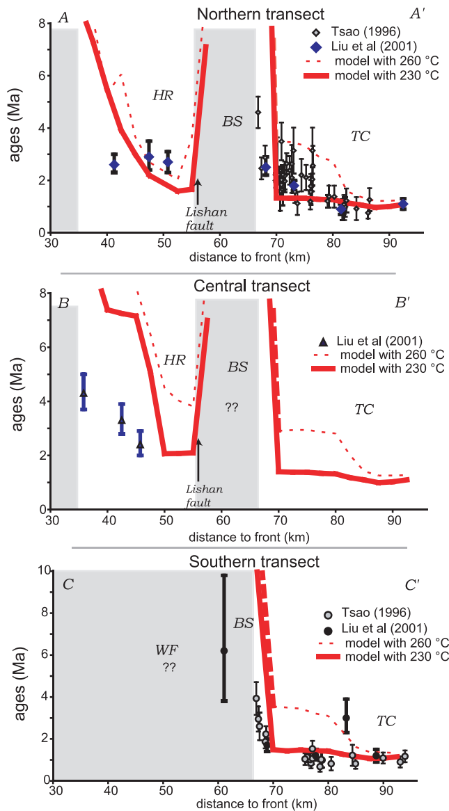
Figure 9. FT ages on detrital zircon from Liu et al. [2001] and Tsao [1996] with 2- \sigma error bars and predictions from our thermokinematic model by assuming a closure temperature of 260°C (dashed red line) and 230°C (solid red line). Pooled ages are taken for the data from Tsao [1996]. In the case of the data from Liu et al. [2001], \chi^2 ages are considered. Shaded areas indicate where the ages are partially reset or nonreset. In the case of the central transect, no data are available for the BS and TC, and we assume that the extent of the area where ages are not reset is similar to that of the northern transect. Also data are not available over the WF of the southern transect, and we suppose that ages may be not reset or only partially reset.
