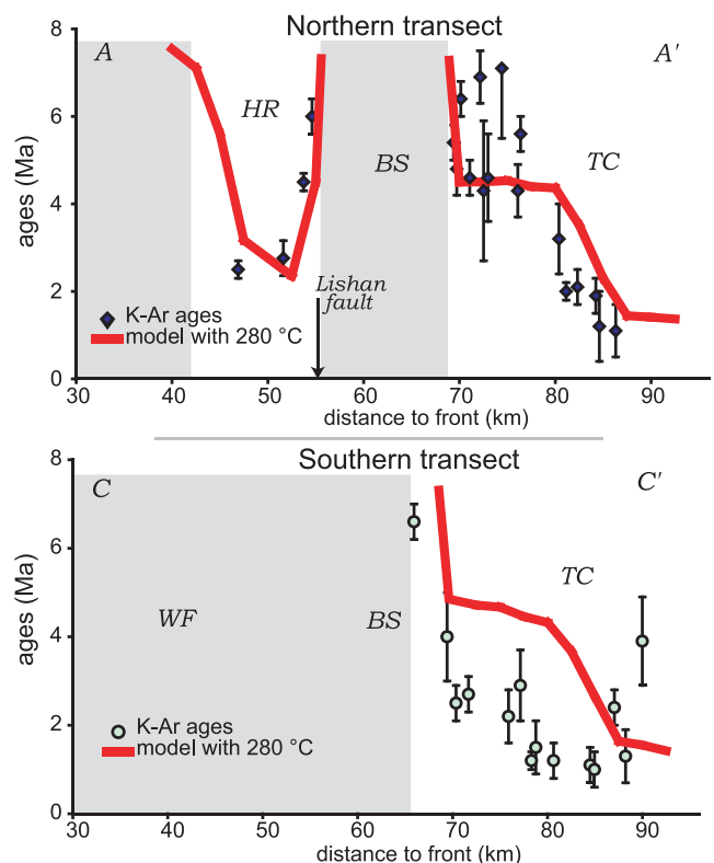
Figure 12. K-Ar ages on white mica fine fractions from Tsao [1996] with 2-σ error bars and predictions of our thermokinematic model assuming a closure temperature of 280°C (red line). Shaded areas locate nonreset ages. In the case of the WF of the southern transect, data are not available to indicate whether or not these ages are reset. The location of nonreset ages drawn here is only supposed by comparison with model predictions.
