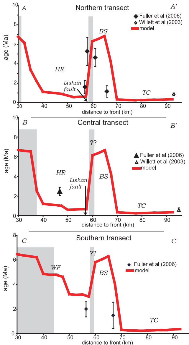
Figure 11. Measured FT ages on apatite [Fuller et al., 2006; Willett et al., 2003] and predictions of our model assuming a closure temperature of 100°C (red line). Shaded areas indicate the regions where ages are not reset. These regions are inferred in the case of the BS of the central and southern transects by comparison with observations from the northern transect and by analogy with what is obtained from other thermochronological ages (Figures 9 and 10).
