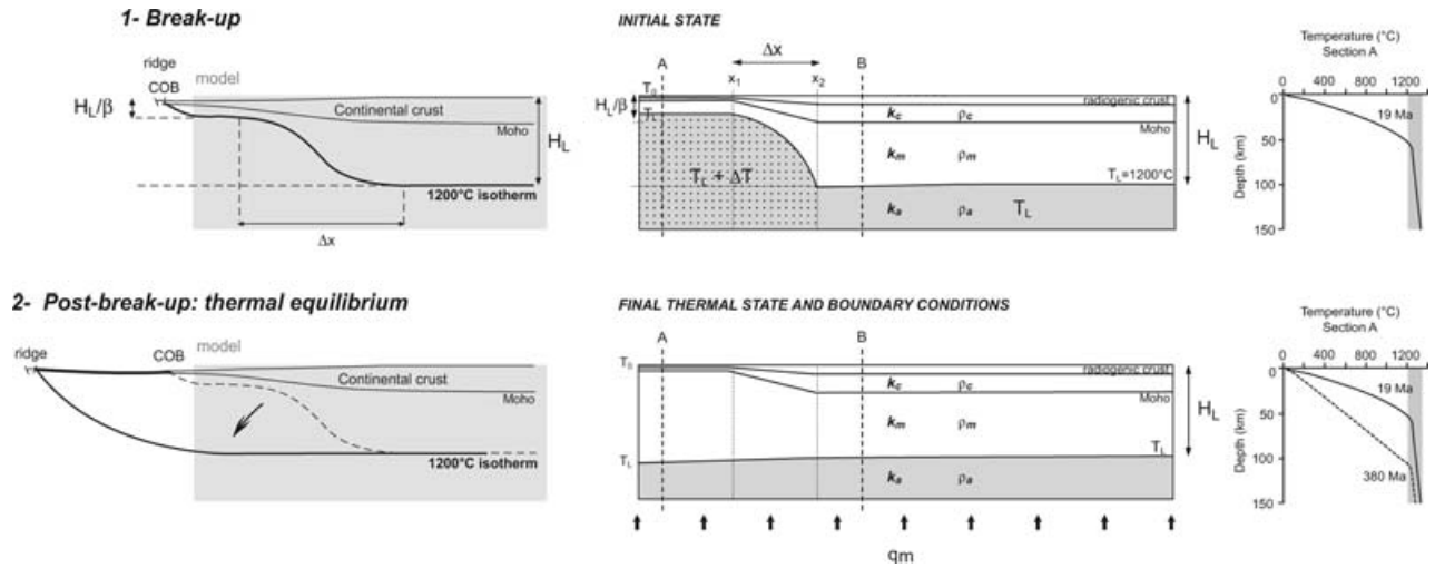
Figure 2. Geometry and thermal structure of a passive margin in nature (left-hand side) and in the numerical model (right-hand side), (1) at the end of continental breakup (initial state) and (2) tens of Ma after drifting, when the lithosphere is thermally re-equilibrated (stable thermal state). The 1200 °C isotherm defines the lithosphere bottom. Its shape under continental part is defined from the initial thermal state, by the stretching factor \beta and value \Delta x . The asthenosphere temperature beneath the stretched part is set to 1200 °C + \Delta T ( \Delta T varying between 0 and 200 °C for different model set up).
