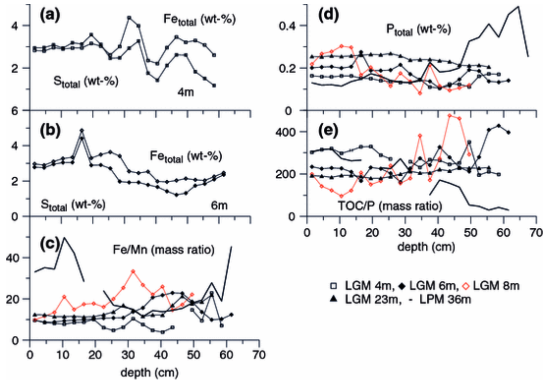
Fig. 7 Geochemical sediment profiles from the centre of LPM and from LGM cores. (a, b) Profiles, showing coincidence between Fe_{total} and S_{total} peaks in the sediment cores 4 m and 6 m from the shallow water area. (c) Fe/Mn fractionation in LPM and LGM. In the steeply inclining sector of the LGM basin, Fe is distinctly enriched versus Mn by precipitation of Fe-oxihydroxides. The dissolved Fe concentrations in the monimolimnion of LPM exceeded 100 mg/l in 1995 (Chiodini et al. 1997); dissolved Fe is precipitated as FeS ; formation of Fe(Mn,Ca) -carbonates is prevented by pH-lowering associated with high CO_2 concentrations in the deep water of the lake. (d, e) P_{total} and TOC/P profiles of LGM sediments document that the burial rate of P in the sediments from the lake centre is higher than that of littoral sediments
