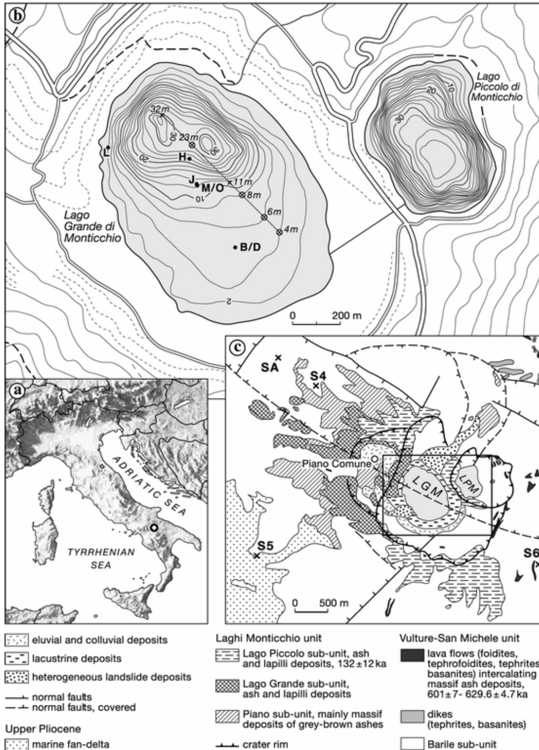
Fig. 1 (a) Location of Laghi di Monticchio. (b) Bathymetry of the maar lakes, map of Lago Grande di Monticchio showing sampling sites for short cores ( \circ ) and in situ pore water profiles ( \times ); locations of piston core records (B, D, J, H, M, O, L) investigated in previous studies are marked inside. (c) Geological map re-drawn after Giannandrea et al. (2004) showing faults, the crater rim of the Monticchio unit and local springs (SA, S4, S5, S6) analyzed by Barbieri and Morotti (2003)
