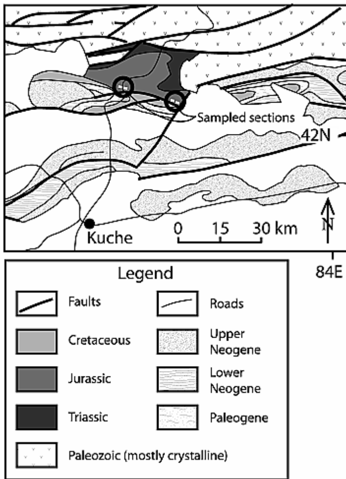
Figure 7. Simplified geologic map of the Kuche area [after Xinjiang Bureau of Geology and Mineral Resources, 1993] (see Figure 1 for regional map).
