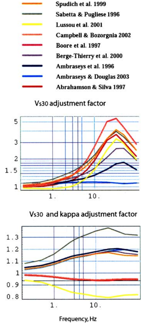
Figure 4. Adjustment factors. (top) V_{s30} adjustment factors using generic rock models. Host region V_{s30} velocities are described in Table 2 (best estimate values). The target velocity is equal to 650 m/s. (bottom) V_{s30} and kappa adjustment factors; host region parameters are described in Table 5. The target kappa value is equal to 0.0125 s.
