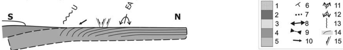
Figure 8. Synthetic map of structural discrepancies in Northern Iceland and schematic cross sections illustrating the different flexure processes. Details, numbered in key, are as follows: 1, flexure zone; 2, active volcanic system; 3, upper Pleistocene–Holocene lava flows (<0.8 Ma); 4, Plio-Pleistocene lava flows (<3.3 Ma and >0.8 Ma); 5, Tertiary lava flows (>3.3 Ma); 6, dip of lava flows; 7, angular unconformity; 8, axis of antiform-like structure; 9, axis of synform-like structure; 10, sense of dip in flexure zone; 11, synform-like structure axis; 12, antiform-like structure axis; 13, angular unconformity; 14, lava flow dip (in cross view); (15), flexural extension. Abbreviations are as follows: ASSH, Antiform-Synform System of Hellisheidi; EA, Eyjafjörður Antiform; EU, Eastern Unconformity; FU, Flateyjarskagi Unconformity; Ho., Hofsjökull; HSS, Húnaflói-Skagi Synform; La., Langjökull; NVZ, Northern Volcanic Zone; SA, Skagaheidi Antiform, SnS, Snaefellsnes; SPRA, Skagafljörður Paleo-Rift Axis; SS, Skagafljörður Synform; U, Unconformity. Note dip variations in flexure zones. Indicative positions for cross sections are indicated by dotted lines. Construction of schematic cross sections is adapted from Bodvarsson and Walker [1964], Daignières et al. [1975], Helgason [1984], and Palmason [1980].
