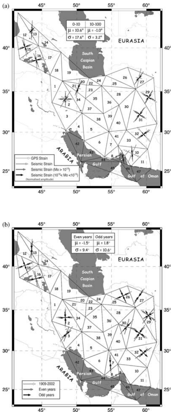
Figure 5. (a) Strain-rate patterns of the seismic data averaged over different seismic moment ranges. Only the styles and the orientations are plotted. Amplitudes are normalized. (b) Strain-rate patterns of the seismic data for the even years and odd years. Amplitudes are normalized. In both figures, the table gives the mean and the standard deviation of the deviation of the direction of the strain obtained using the subsets of data respectively to the whole set of data.
