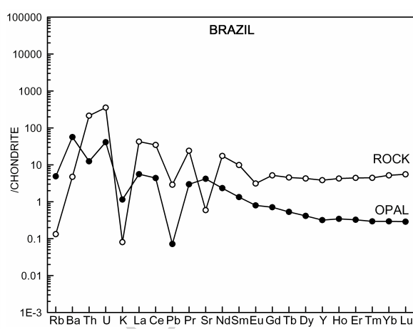
Figure 6: Multi-element diagram of a Brazilian opal compared to its sandstone host rock normalized to chondrite (couple n° 766). The two patterns are near parallel, except for Rb, Ba, K, Sr, which are more concentrated in opal. Depletion in HREE compared to LREE is explained by a lesser mobility of HREE, which stay preferentially in the rock during weathering.
