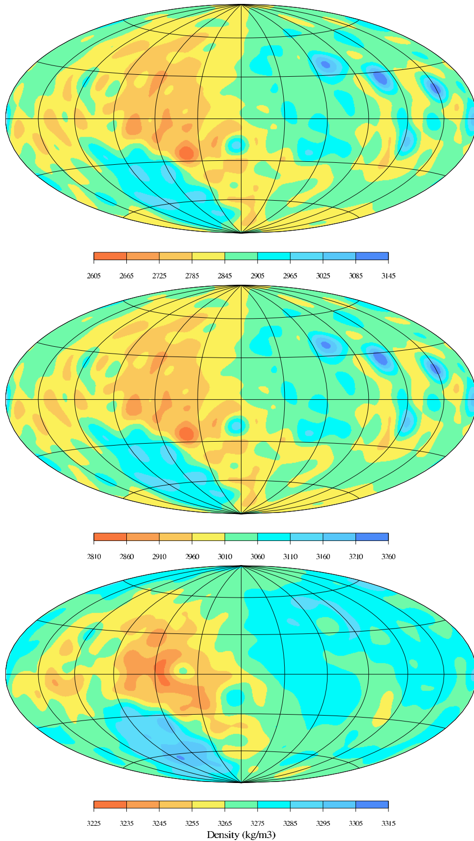
Figure 6. Density \delta_{\phi\rho} ( \text{kg/m}^3 ) (top) at the moon surface, (middle) at the bottom of the crust (40 km depth), and (bottom) in the upper mantle (100 km depth). The projection is the same as for Figure 5.
