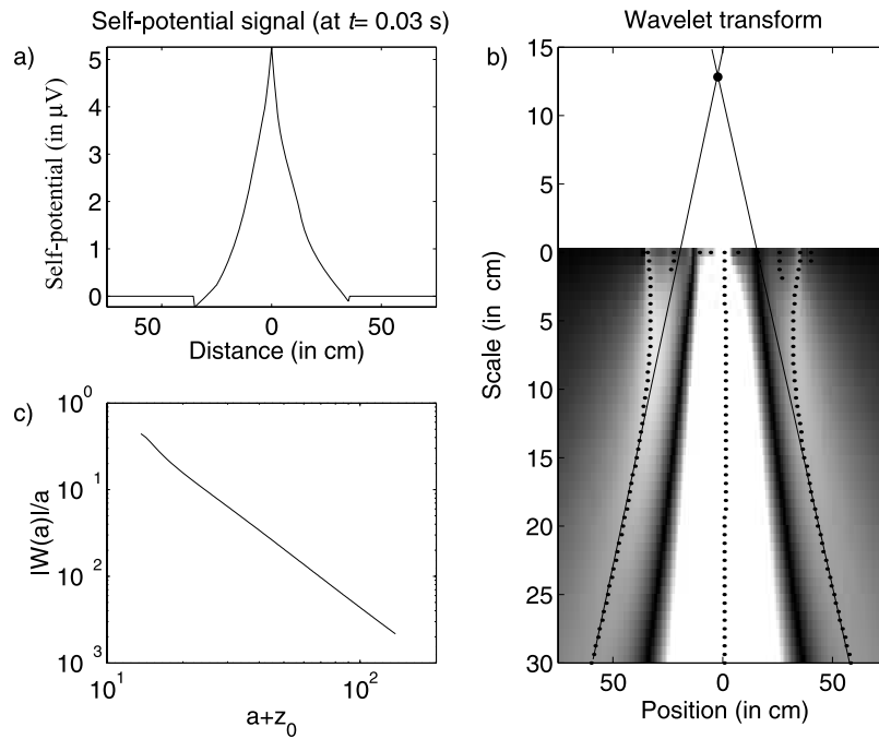
Figure 18. Wavelet analysis of the self-potential data at the maximum development of the self-potential anomaly in the case of the pulse pumping of water. (a) Measured self-potential signals in \mu V . (b) Continuous wavelet transform using a first order vertical wavelet. The solid lines show the wavelet coefficient maxima that intersect at the position of the source. (c) The order of the source is estimated from the slope of |W(a)|/a versus a + z_0 . The source corresponds to an electrical dipole.
