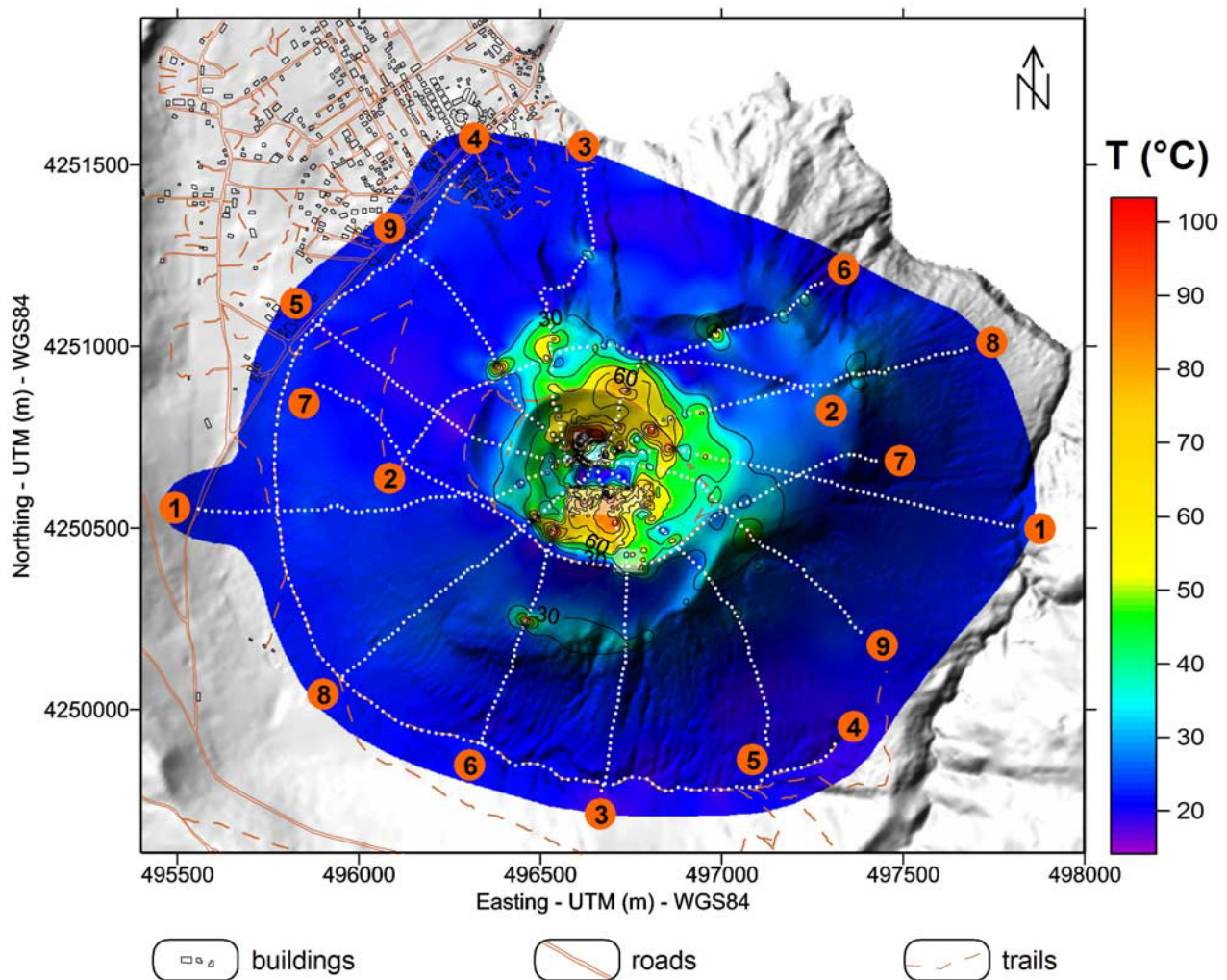
Figure 8. Map of the temperature at a depth of 30 cm superimposed on the DEM of La Fossa cone. The white dots correspond to the location of the temperature measurements of the present study. The dots inside the La Fossa crater correspond to the detailed temperature survey (at the same depth of 30 cm) reported by Aubert et al. [2008]. Note that the bottom of the crater is cold (<30°C). Thermal anomalies are sometimes observed on the flanks of the volcano. In this case these anomalies are indicative of the boundaries of ancient craters.
