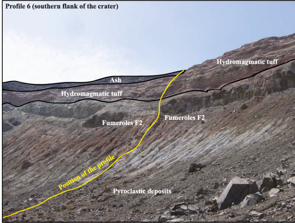
Figure 13. Architecture of the southern part of the crater along profile 6 with the position of the fumerole 2 (F2).
